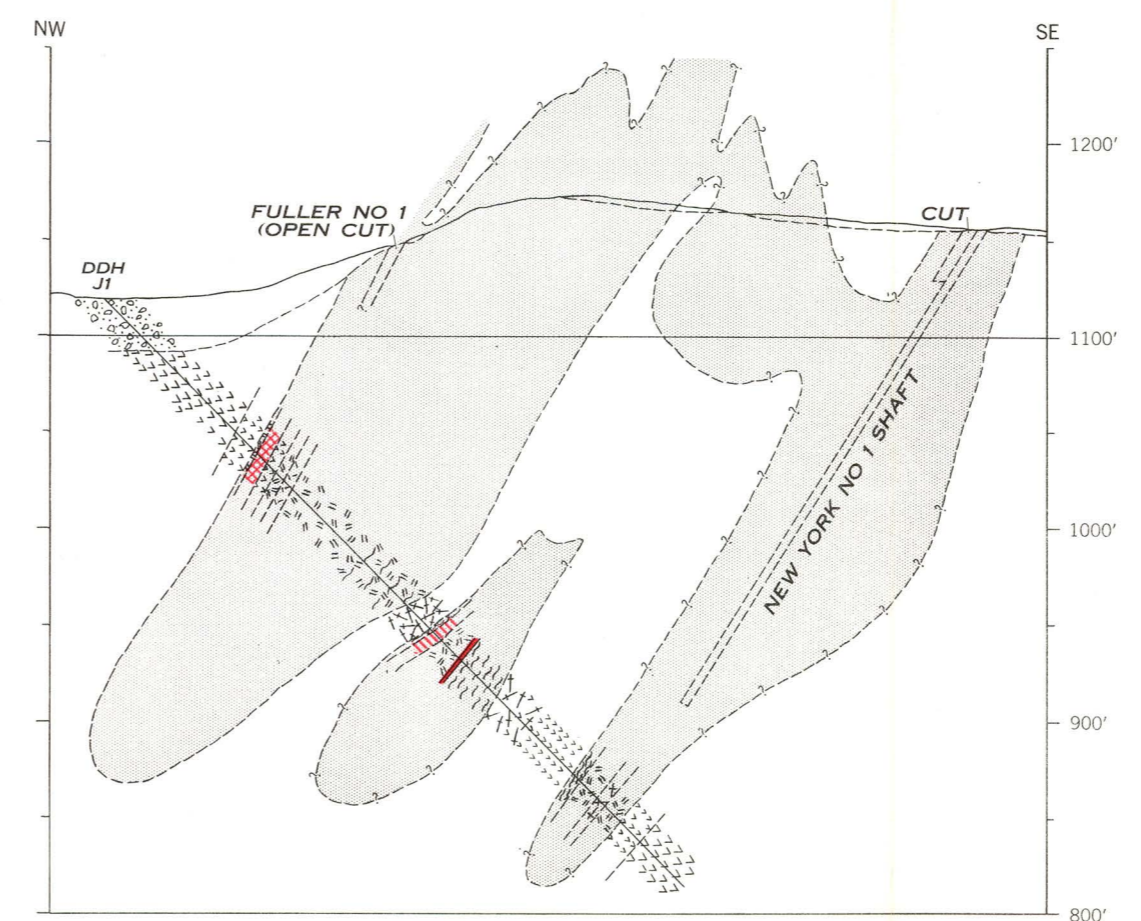
BEDROCK GEOLOGIC AND MAGNETIC MAP AND GEOLOGIC SECTIONS, JAYVILLE DEPOSIT, WEST-CENTRAL RECTANGLE, OSWEGATCHIE QUADRANGLE, ST. LAWRENCE COUNTY, NEW YORK
