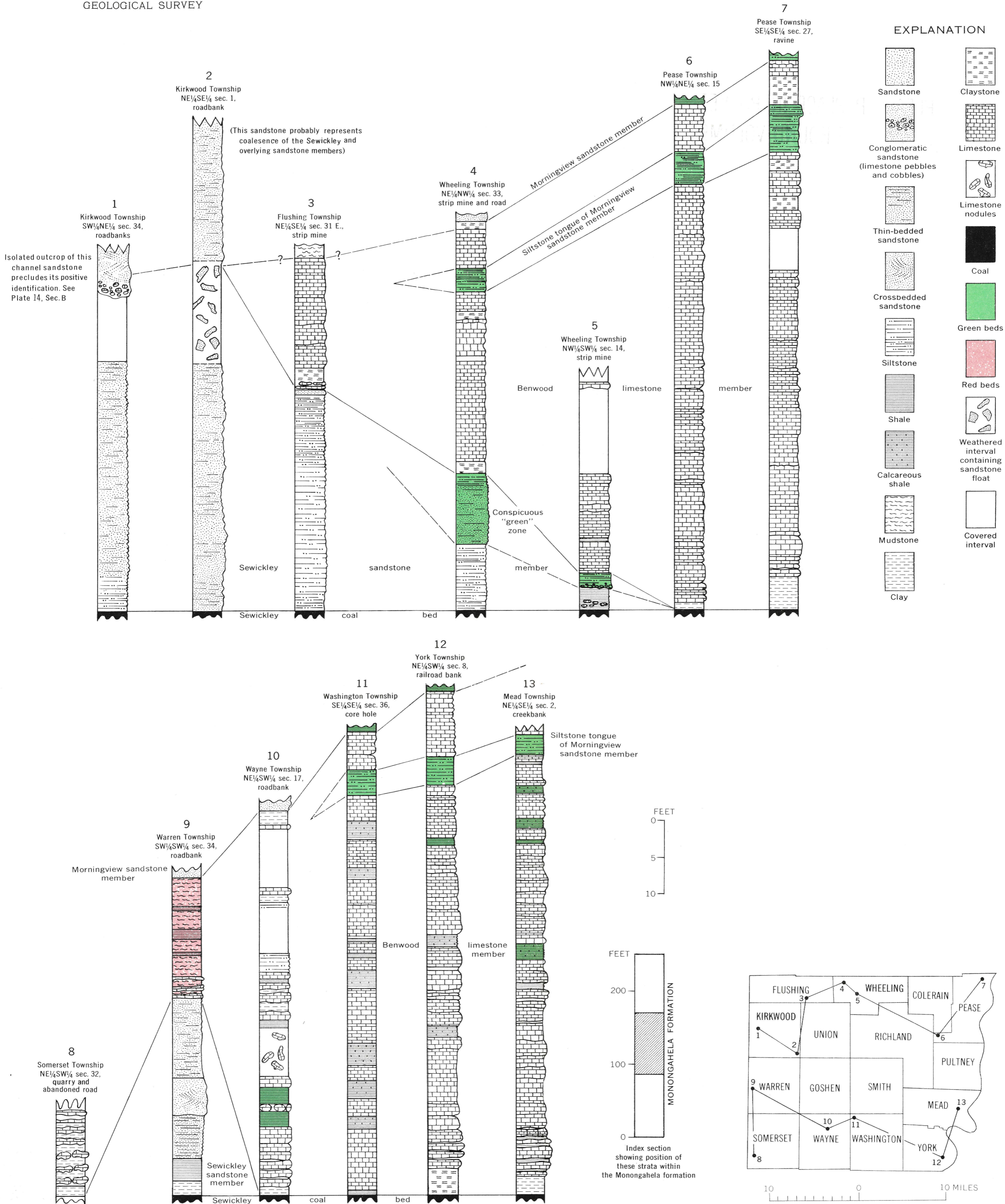
COLUMNAR SECTIONS SHOWING THE STRATIGRAPHIC RELATION OF THE SEWICKLEY COAL BED AND THE SEWICKLEY SANDSTONE, BENWOOD LIMESTONE, AND MORNINGVIEW SANDSTONE MEMBERS OF THE MONONGAHELA FORMATION IN BELMONT COUNTY, OHIO
