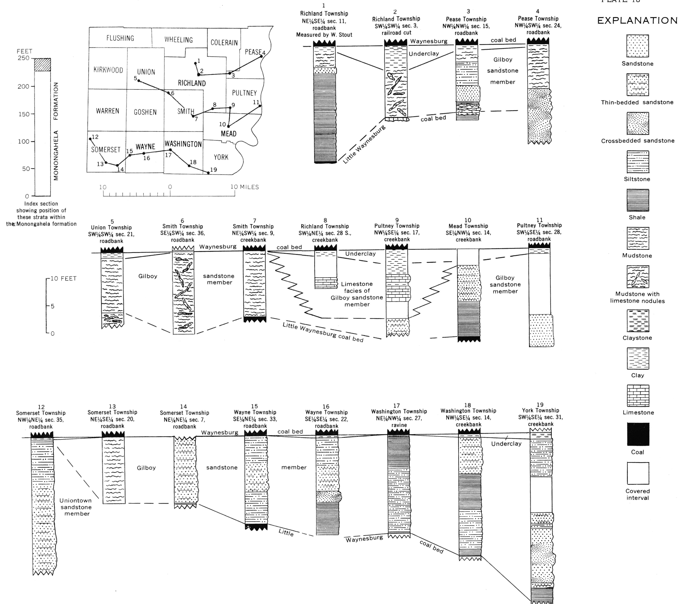
COLUMNAR SECTIONS SHOWING THE STRATIGRAPHIC RELATION OF THE LITTLE WAYNESBURG AND WAYNESBURG COAL BEDS AND THE GILBOY SANDSTONE MEMBER OF THE MONONGAHELA FORMATION IN BELMONT COUNTY, OHIO
