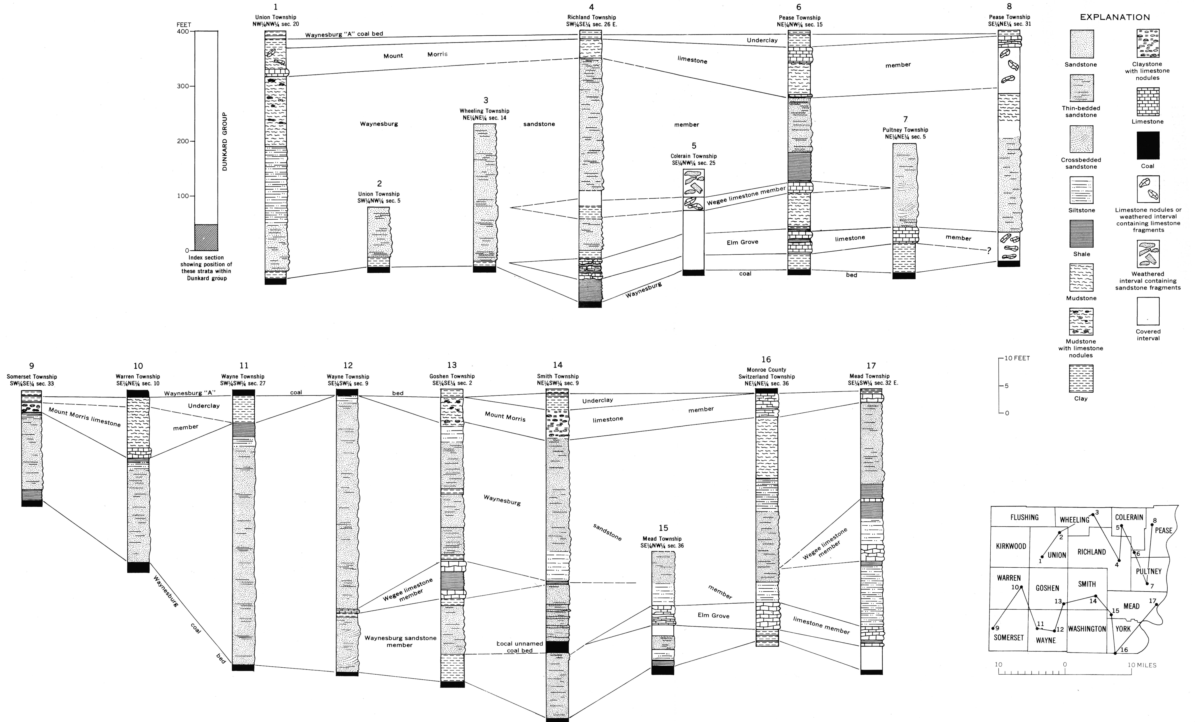
COLUMNAR SECTIONS SHOWING THE STRATIGRAPHIC RELATION OF THE WAYNESBURG AND WAYNESBURG "A" COAL BEDS AND THE ELM GROVE LIMESTONE, WEGEE LIMESTONE, WAYNESBURG SANDSTONE, AND MOUNT MORRIS LIMESTONE MEMBERS OF THE DUNKARD GROUP IN BELMONT COUNTY, OHIO
