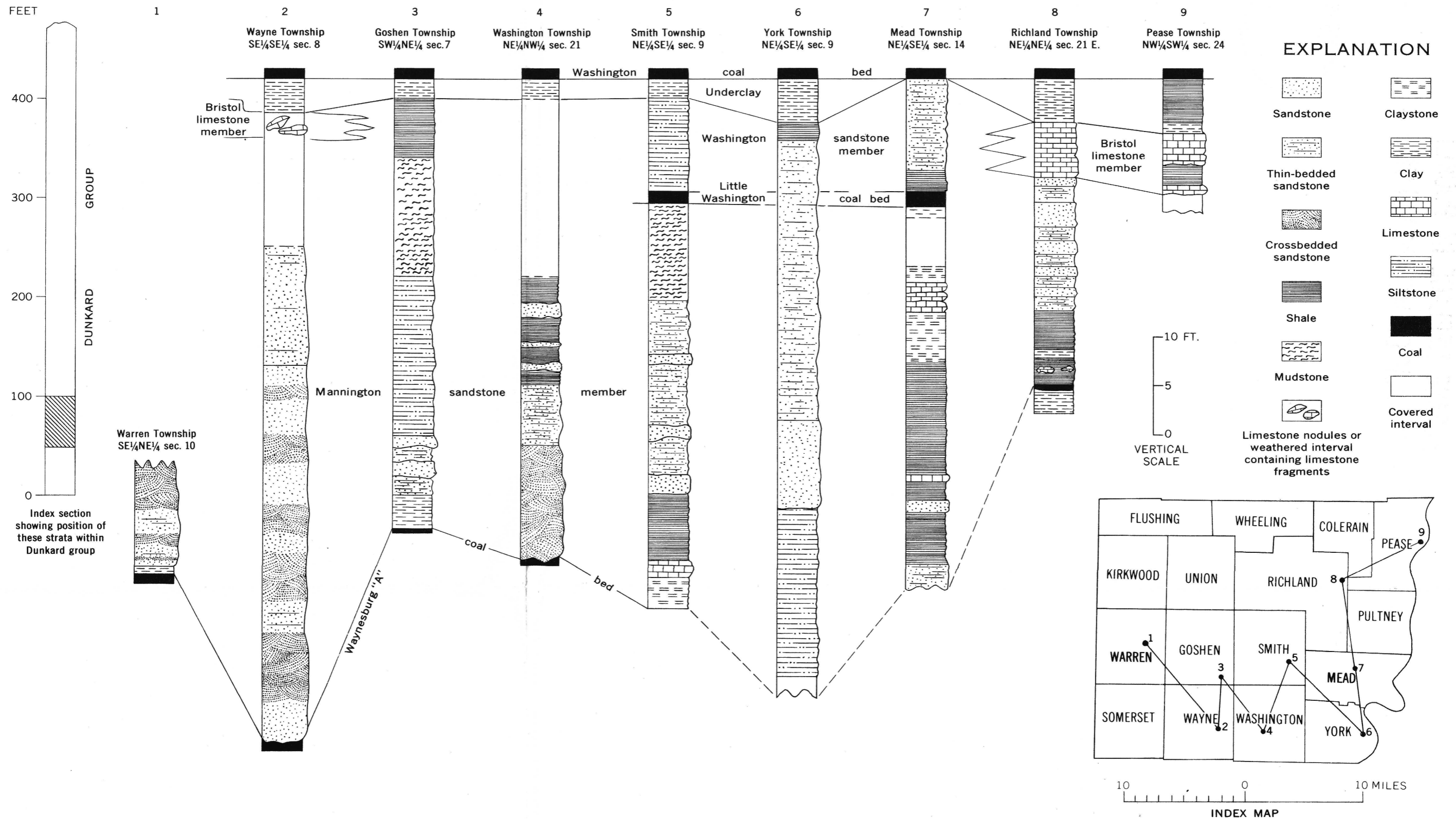
COLUMNAR SECTIONS SHOWING THE STRATIGRAPHIC RELATION OF THE WAYNESBURG "A", LITTLE WASHINGTON, AND WASHINGTON COAL BEDS AND THE MANNINGTON SANDSTONE, WASHINGTON SANDSTONE, AND BRISTOL LIMESTONE MEMBERS OF THE DUNKARD GROUP IN BELMONT COUNTY, OHIO
