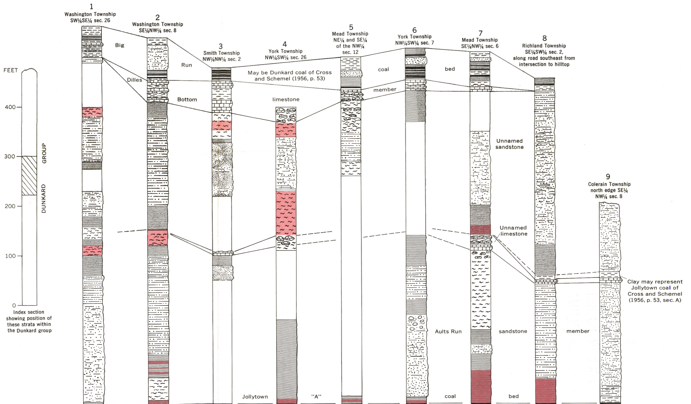
COLUMNAR SECTIONS SHOWING THE STRATIGRAPHIC RELATION OF THE JOLLYTOWN "A" AND BIG RUN COAL BEDS AND THE AULTS RUN SANDSTONE AND DILLES BOTTOM LIMESTONE MEMBERS OF THE DUNKARD GROUP IN BELMONT COUNTY, OHIO
