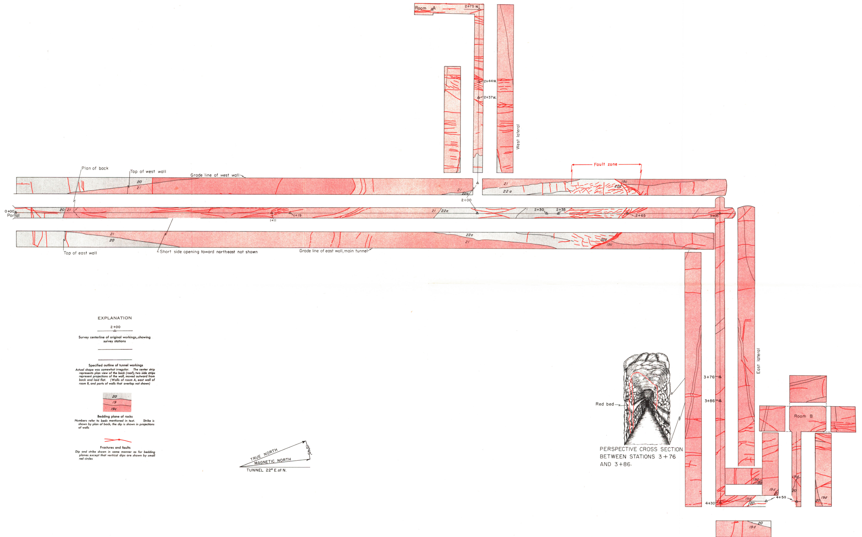
GEOLOGIC MAP OF THE USGS TUNNEL PRIOR TO THE HIGH-EXPLOSIVE TESTS, NEVADA TEST SITE
