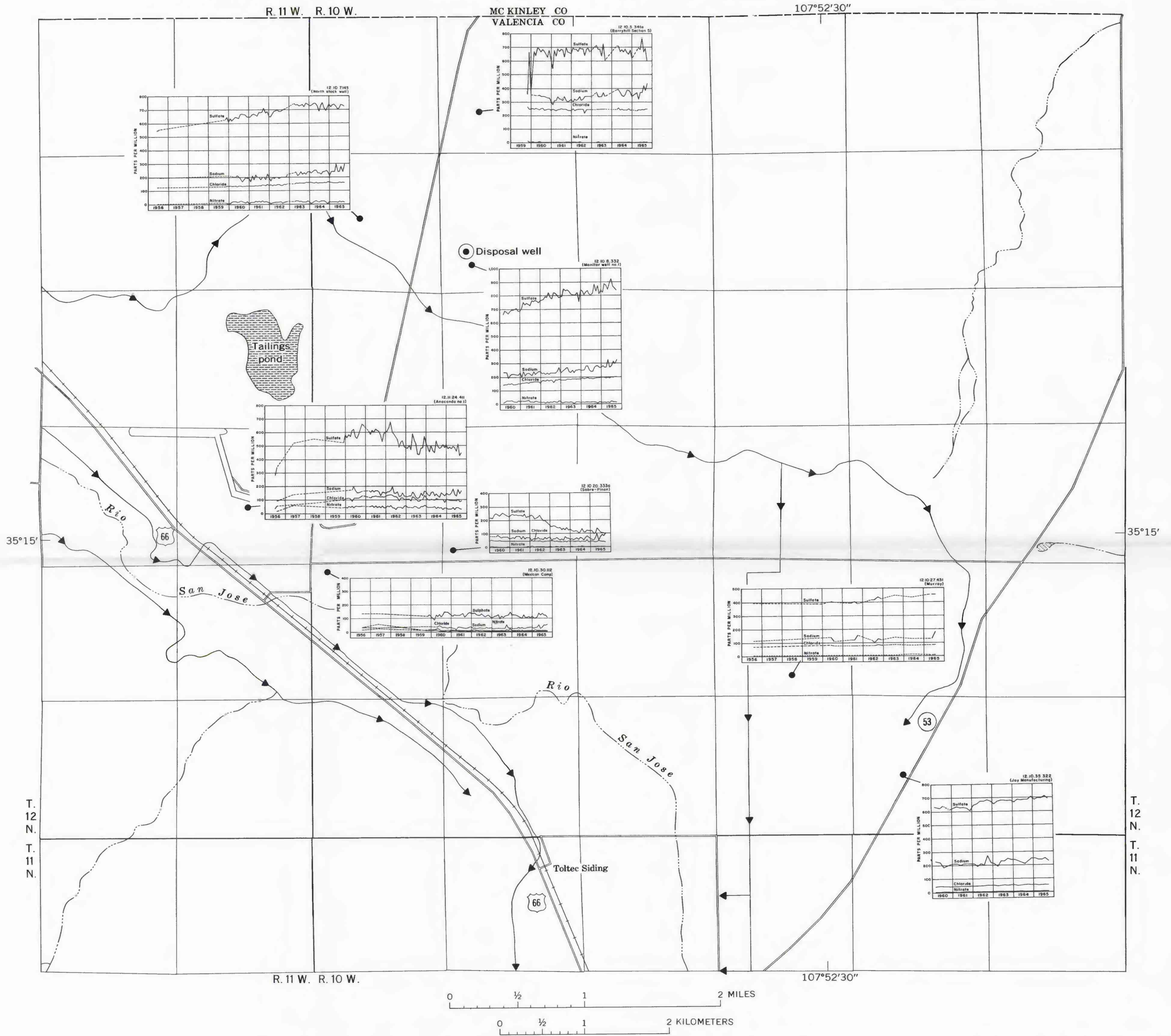
GRAPHS SHOWING CONCENTRATIONS OF SODIUM, SULFATE, CHLORIDE, AND NITRATE IONS IN WATER FROM EIGHT WELLS IN THE VICINITY OF THE ANACONDA CO. TAILINGS POND AND DISPOSAL WELL 1, GRANTS AREA, VALENCIA COUNTY, NEW MEXICO
