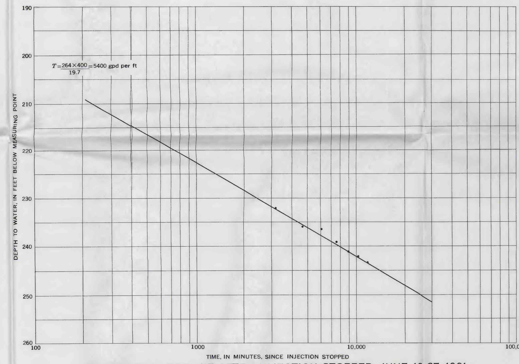
WATER-LEVEL DECLINE AFTER INJECTION STOPPED JUNE 18-27, 1961
