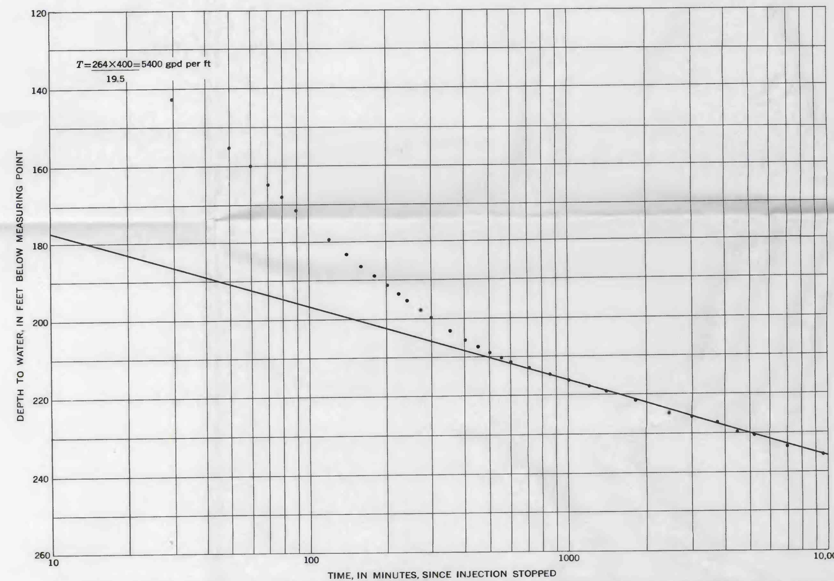
WATER-LEVEL DECLINE AFTER INJECTION STOPPED JANUARY 31 TO FEBRUARY 7, 1961
