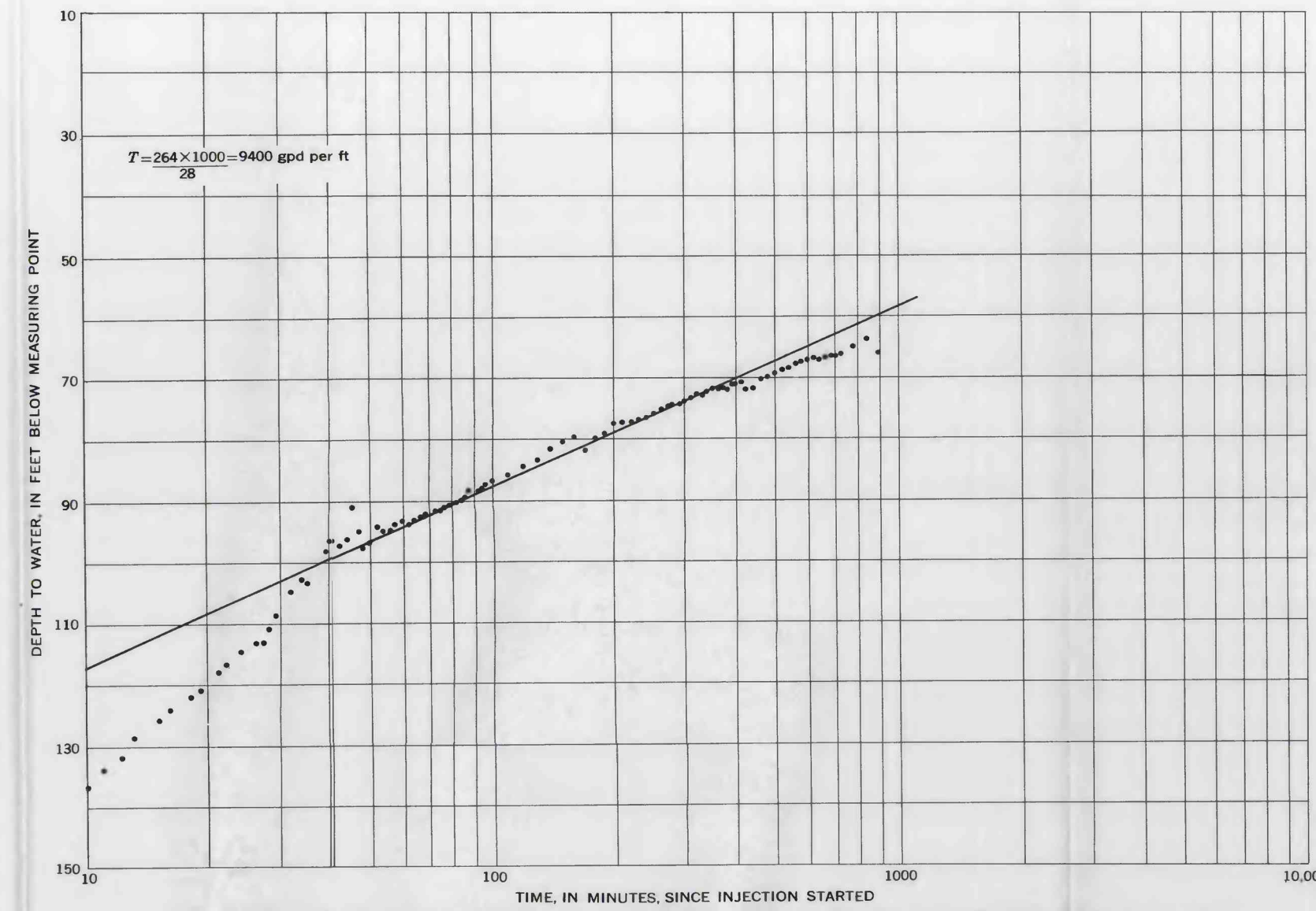
WATER-LEVEL RISE FROM INJECTION, JANUARY 22 TO FEBRUARY 5, 1960
