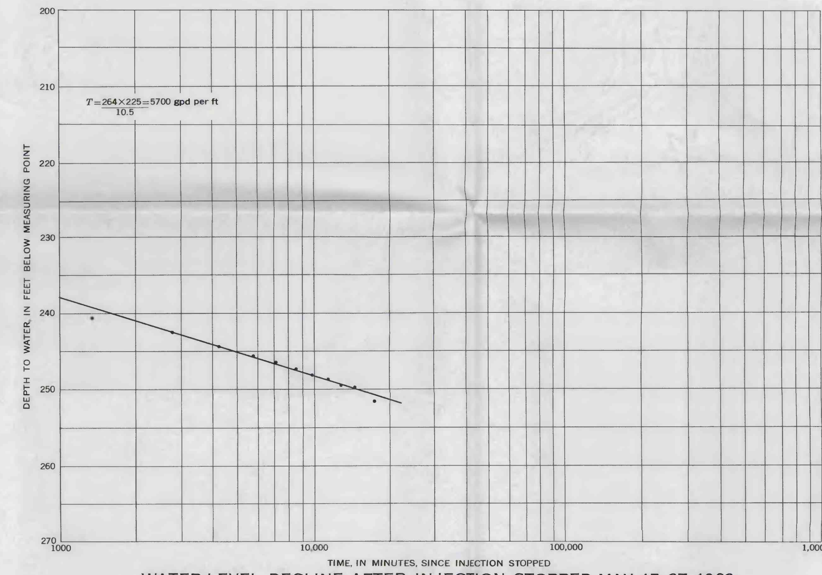
WATER-LEVEL DECLINE AFTER INJECTION STOPPED MAY 15-27, 1962
