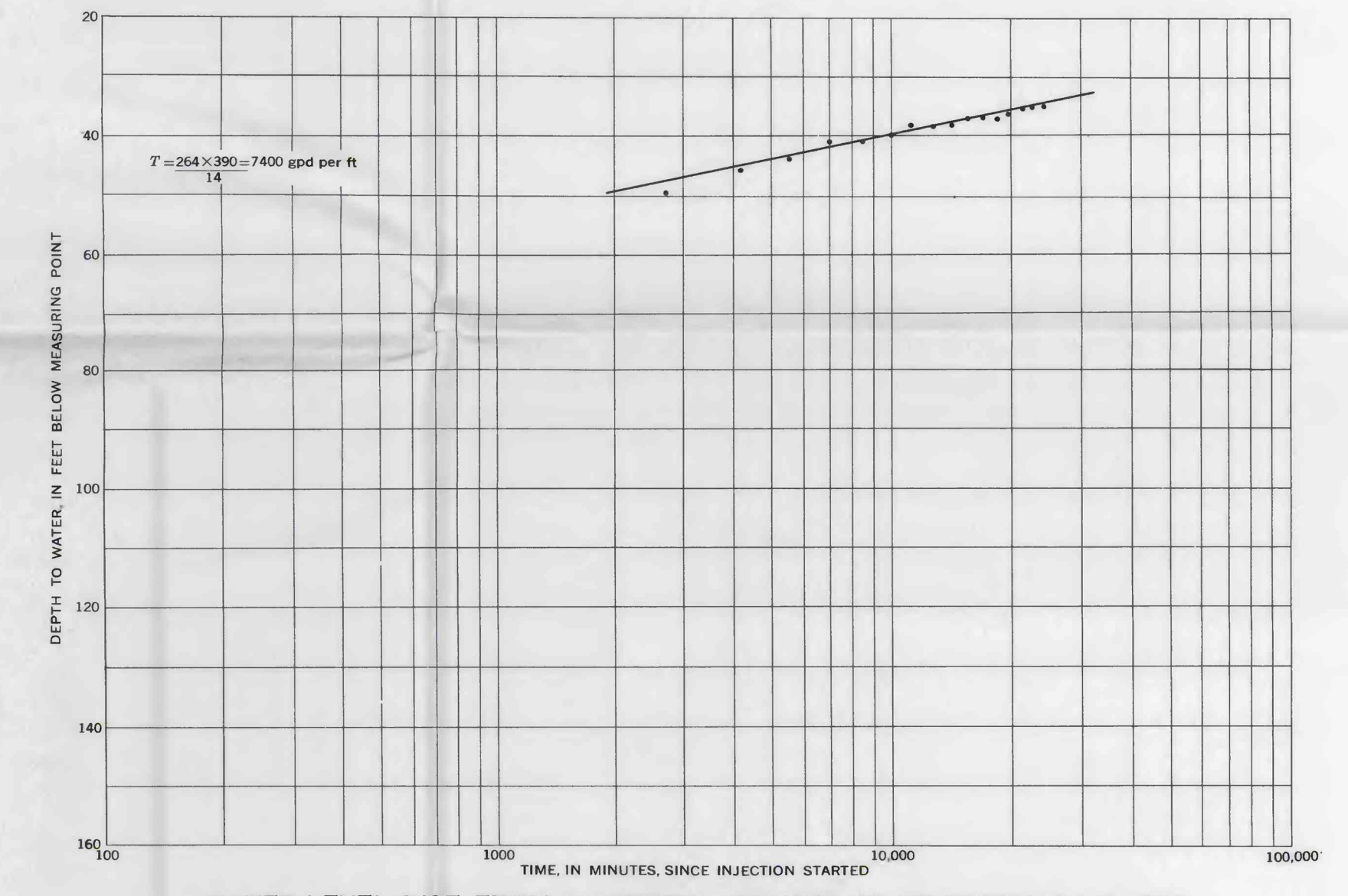
WATER-LEVEL RISE FROM INJECTION, JANUARY 23 TO FEBRUARY 9, 1963
