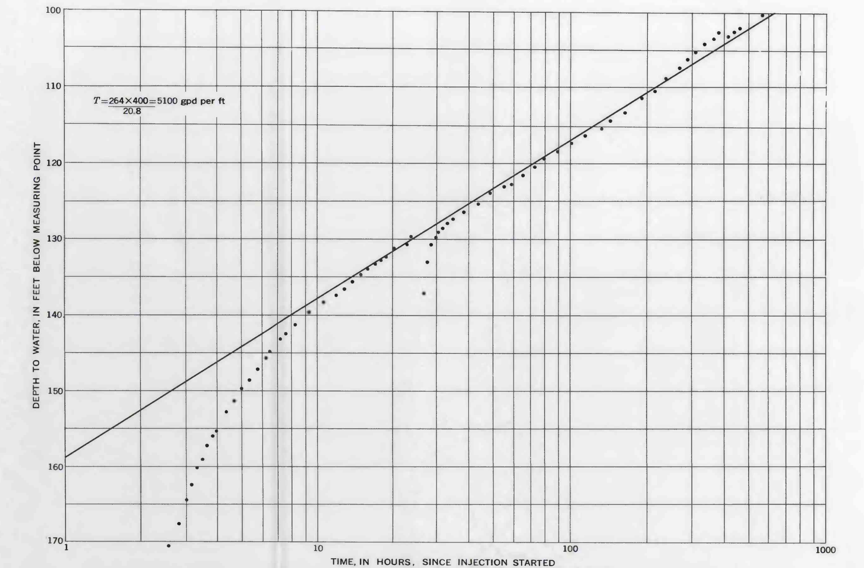
WATER-LEVEL RISE FROM INJECTION, DECEMBER 14, 1960 TO JANUARY 6, 1961
