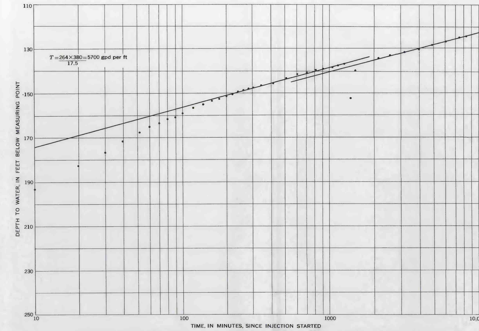
WATER-LEVEL RISE FROM INJECTION, FEBRUARY 28 TO MARCH 14, 1960
