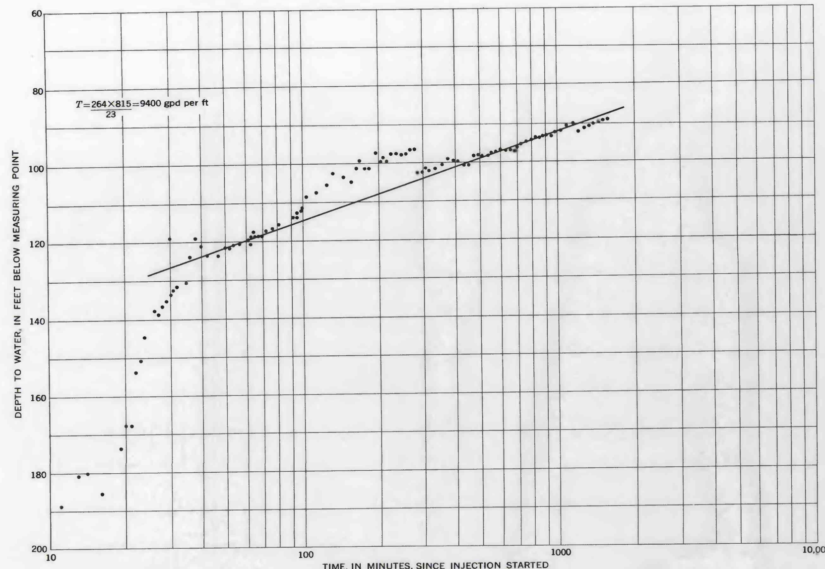
WATER-LEVEL RISE FROM INJECTION, JANUARY 20-21, 1960
