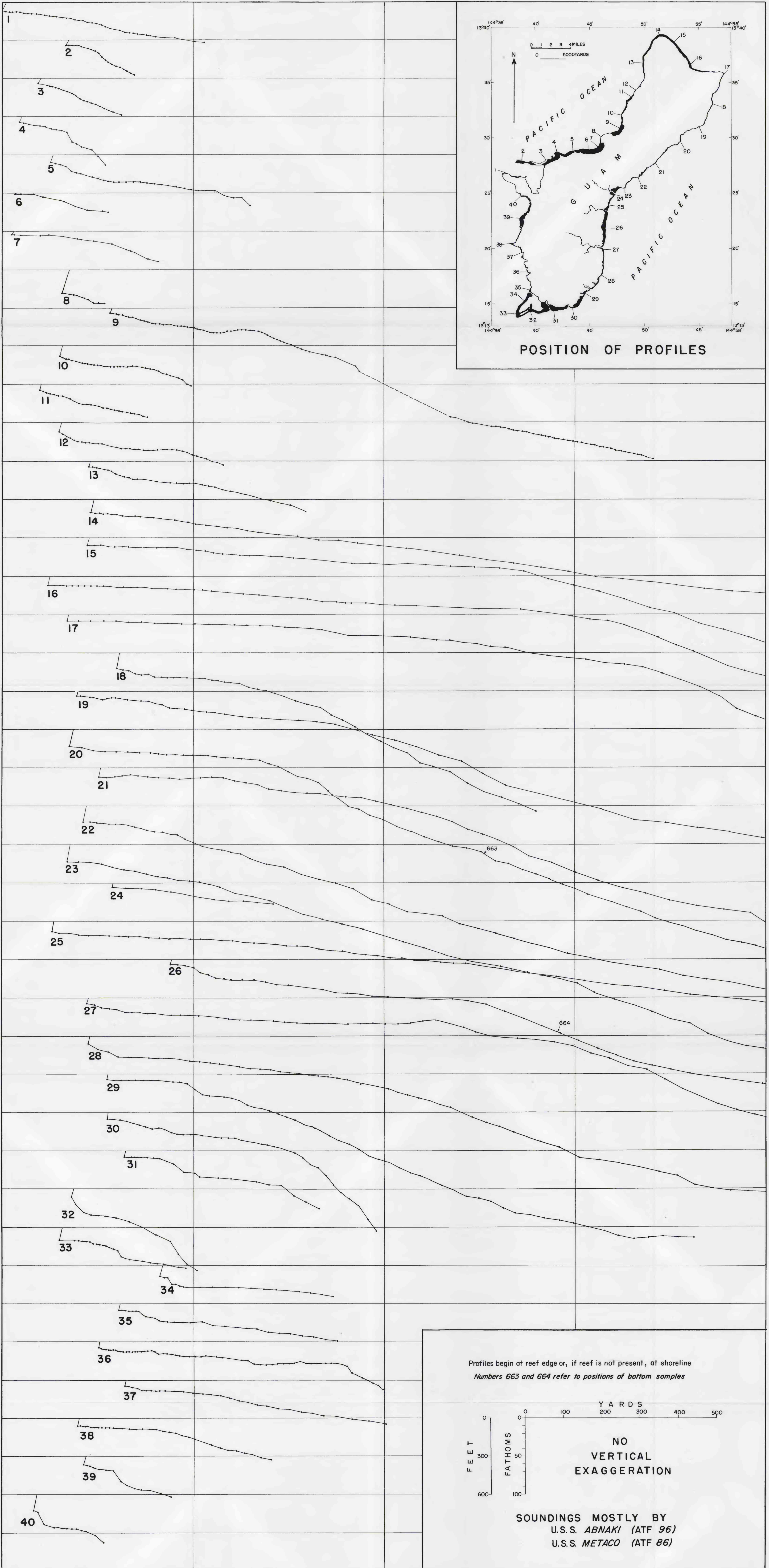
PROFILES OF UPPER SLOPES FRINGING GUAM
