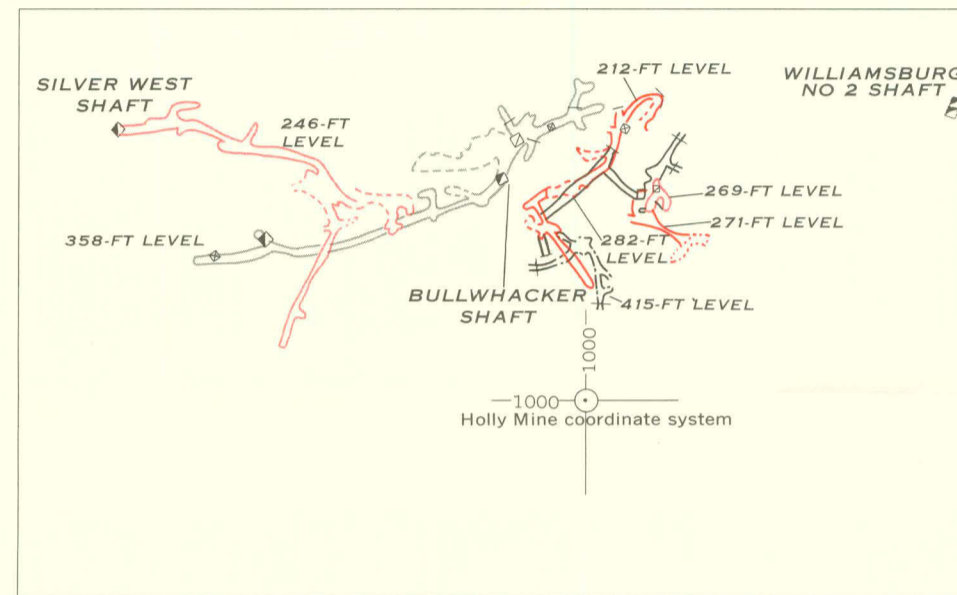
SILVER WEST MINE WORKINGS AND LOWER LEVELS FROM BULLWHACKER SHAFT
