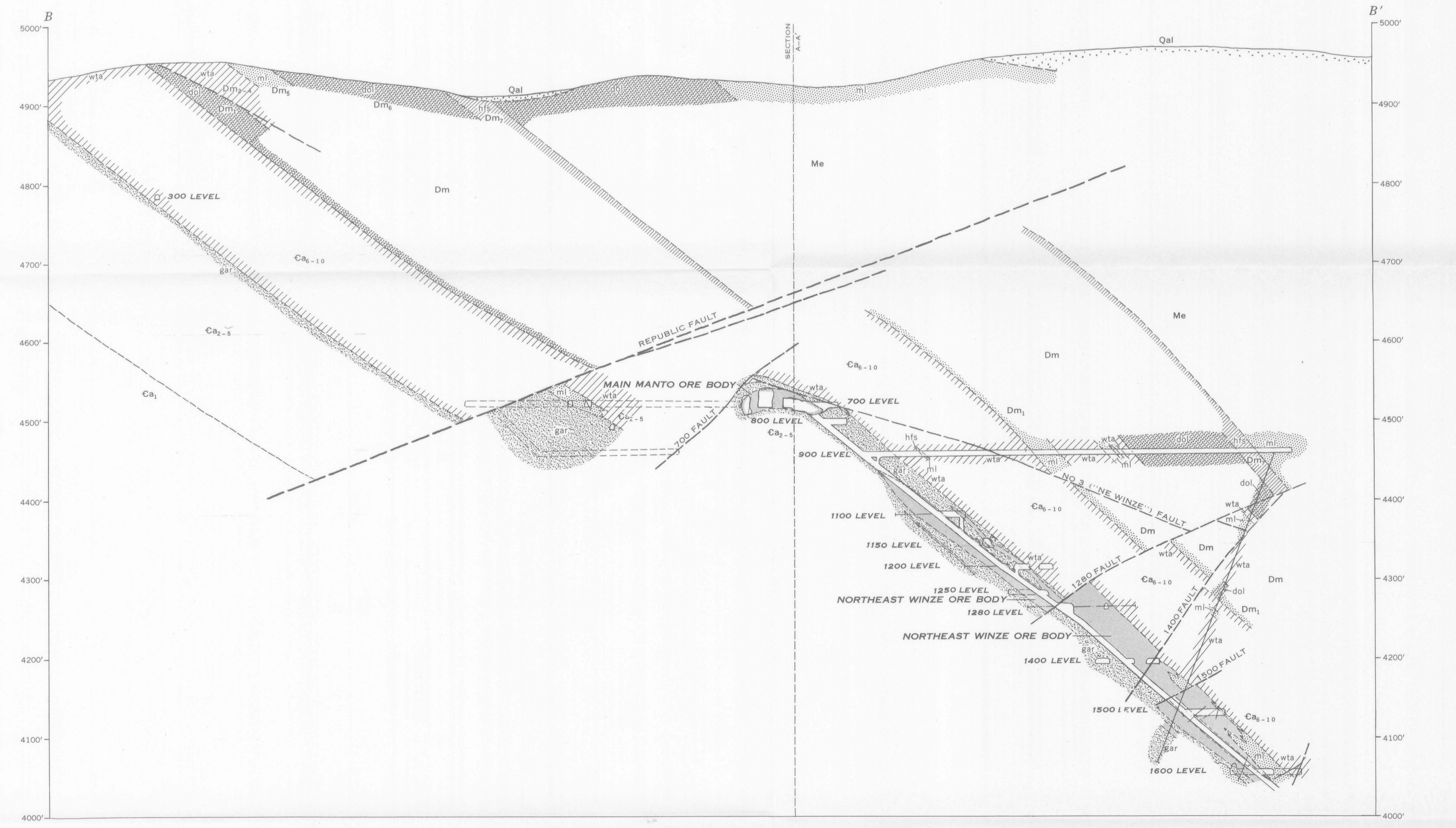
B-B', THROUGH NORTHEAST WINZE
