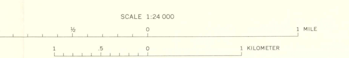
GEOLOGIC STRUCTURE SECTIONS B-B' THROUGH H-H', LA HABRA AND WHITTIER QUADRANGLES, CALIFORNIA
