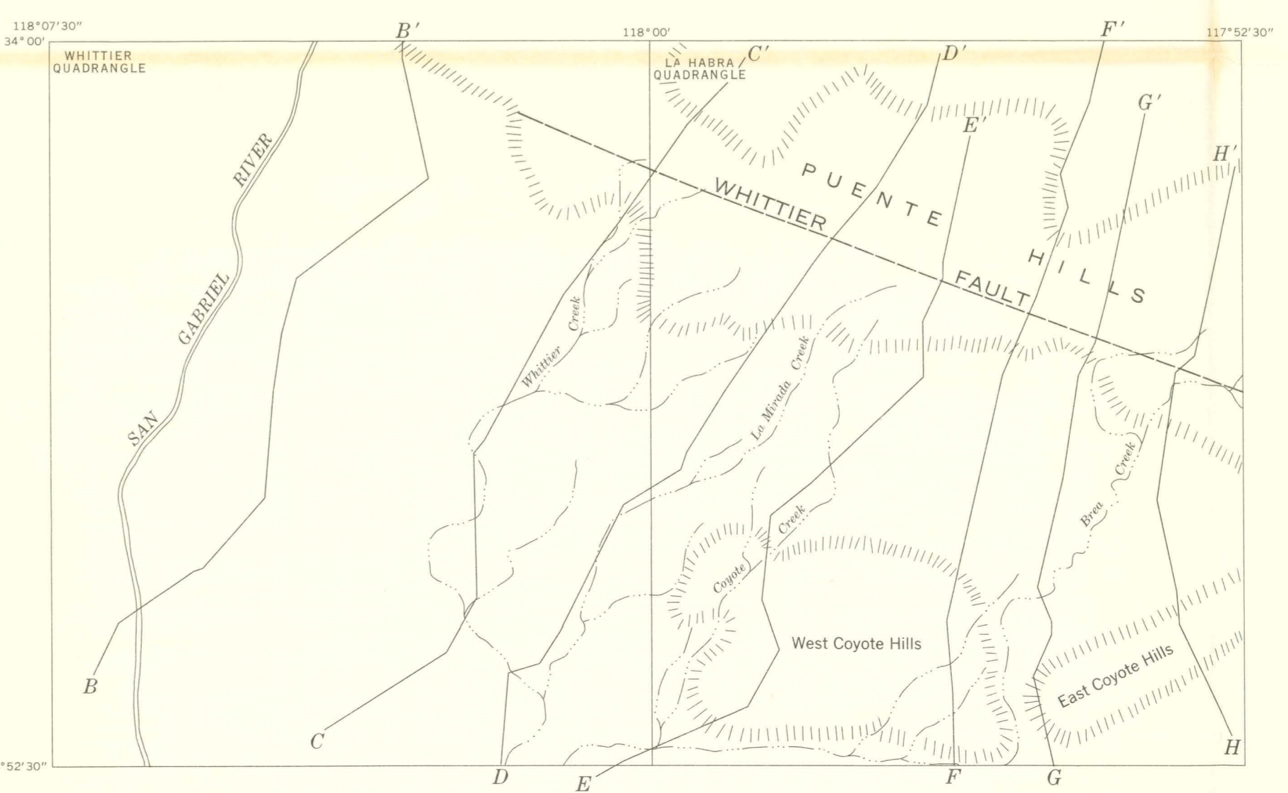
INDEX MAP SHOWING LOCATIONS OF GEOLOGIC STRUCTURE SECTIONS B-B' THROUGH H-H'
