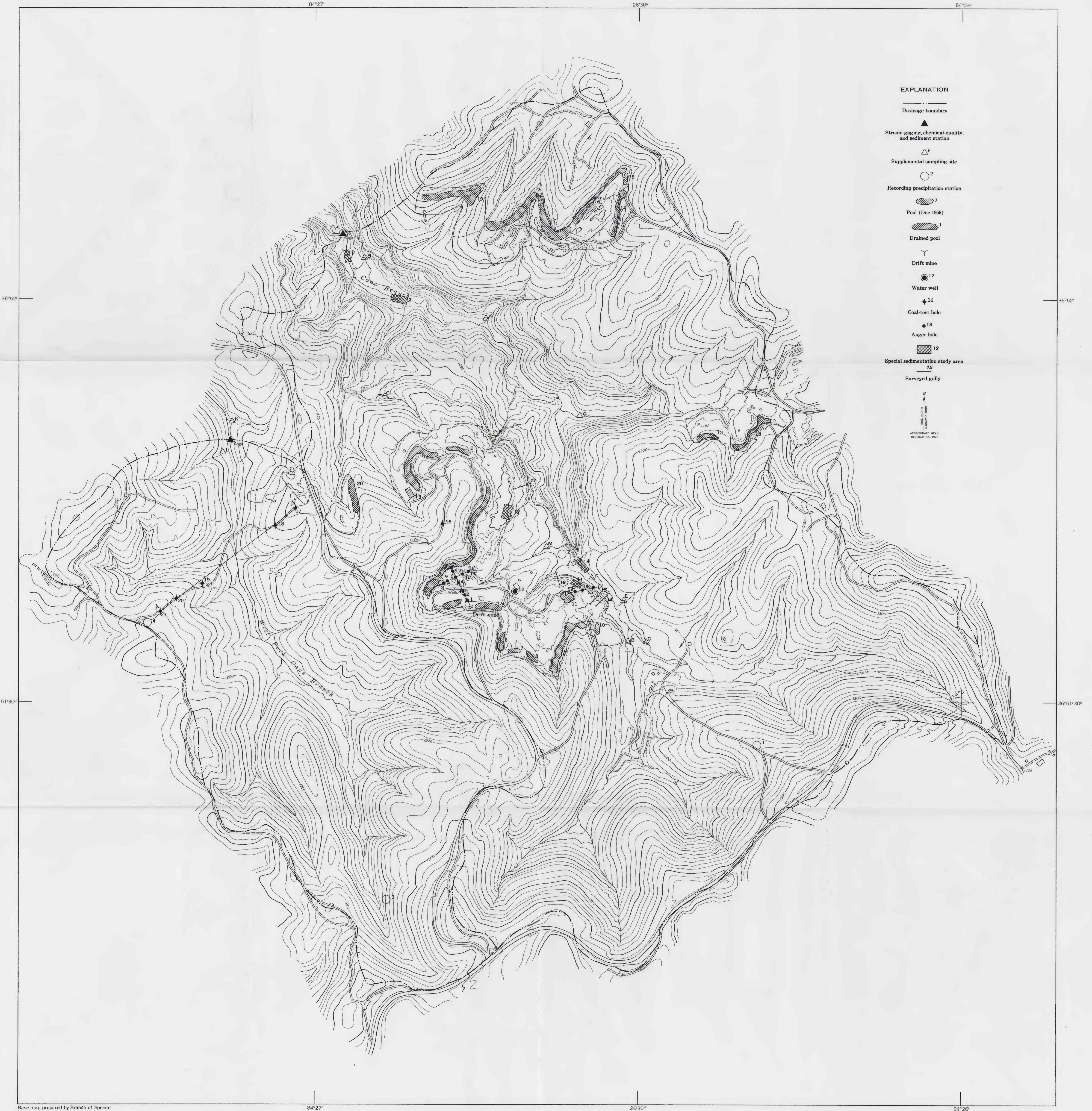
MAP OF CANE BRANCH AND WEST FORK CANE BRANCH STUDY AREAS, KENTUCKY, SHOWING POINTS OF COLLECTION OF HYDROLOGIC DATA
