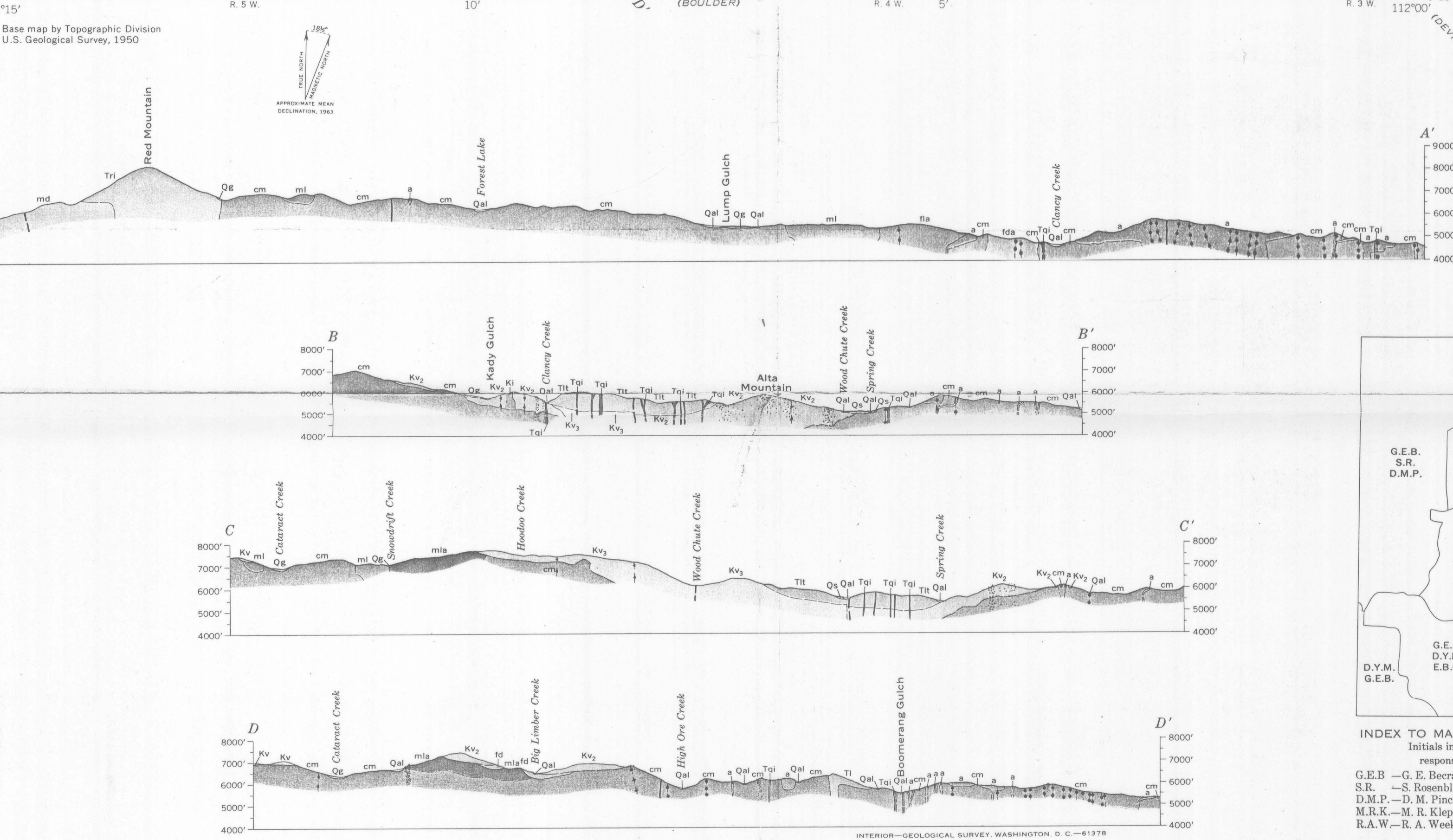
GEOLOGIC MAP AND SECTIONS OF THE JEFFERSON CITY QUADRANGLE, MONTANA, SHOWING LOCATION OF MINES AND PROSPECTS
