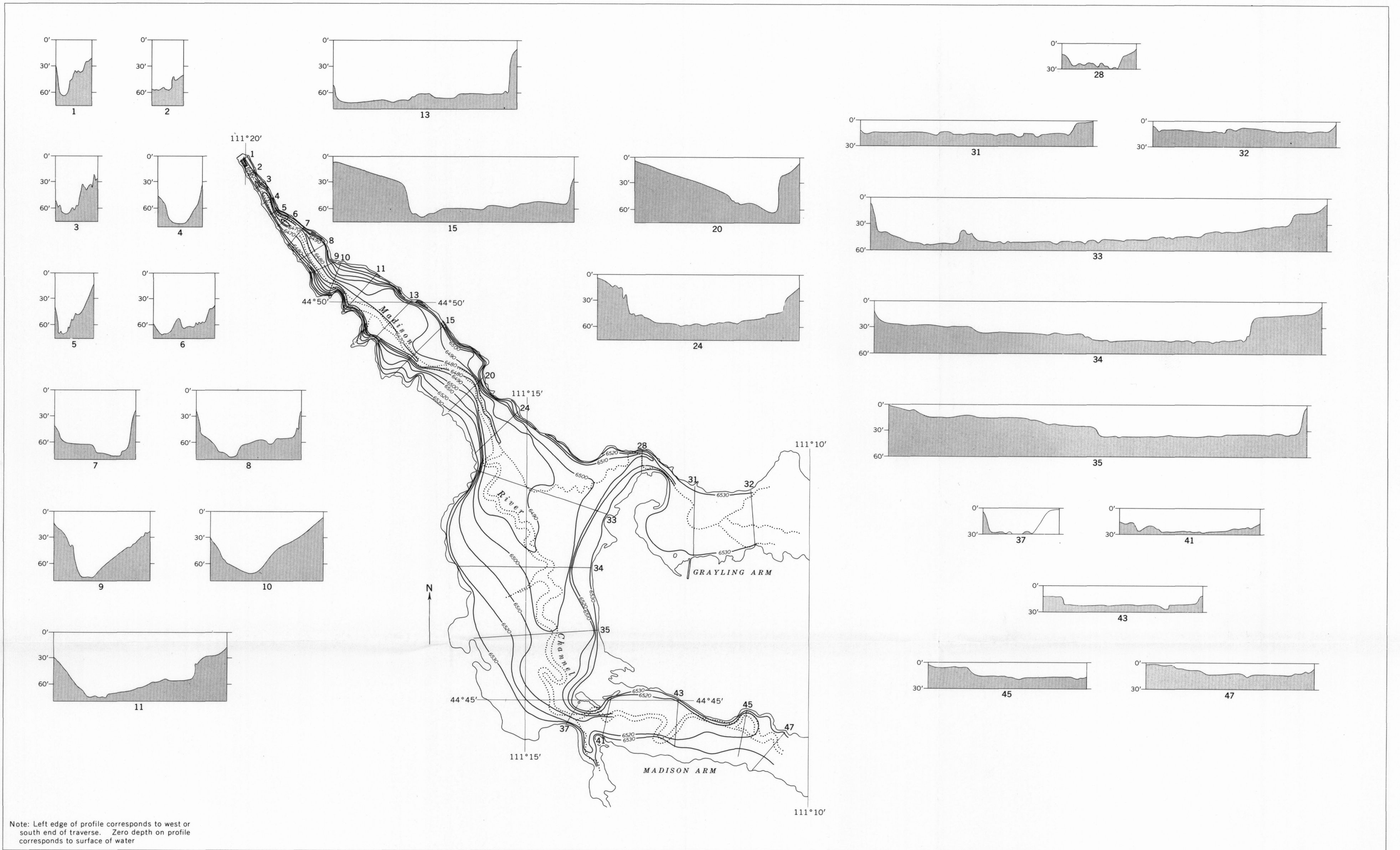
MAP OF HEBGEN LAKE, MONTANA, SHOWING THE LOCATION OF SELECTED DEPTH-SOUNDING TRAVERSES MADE IN SEPTEMBER 1959 AND CORRESPONDING PROFILES OF THE LAKE BOTTOM
