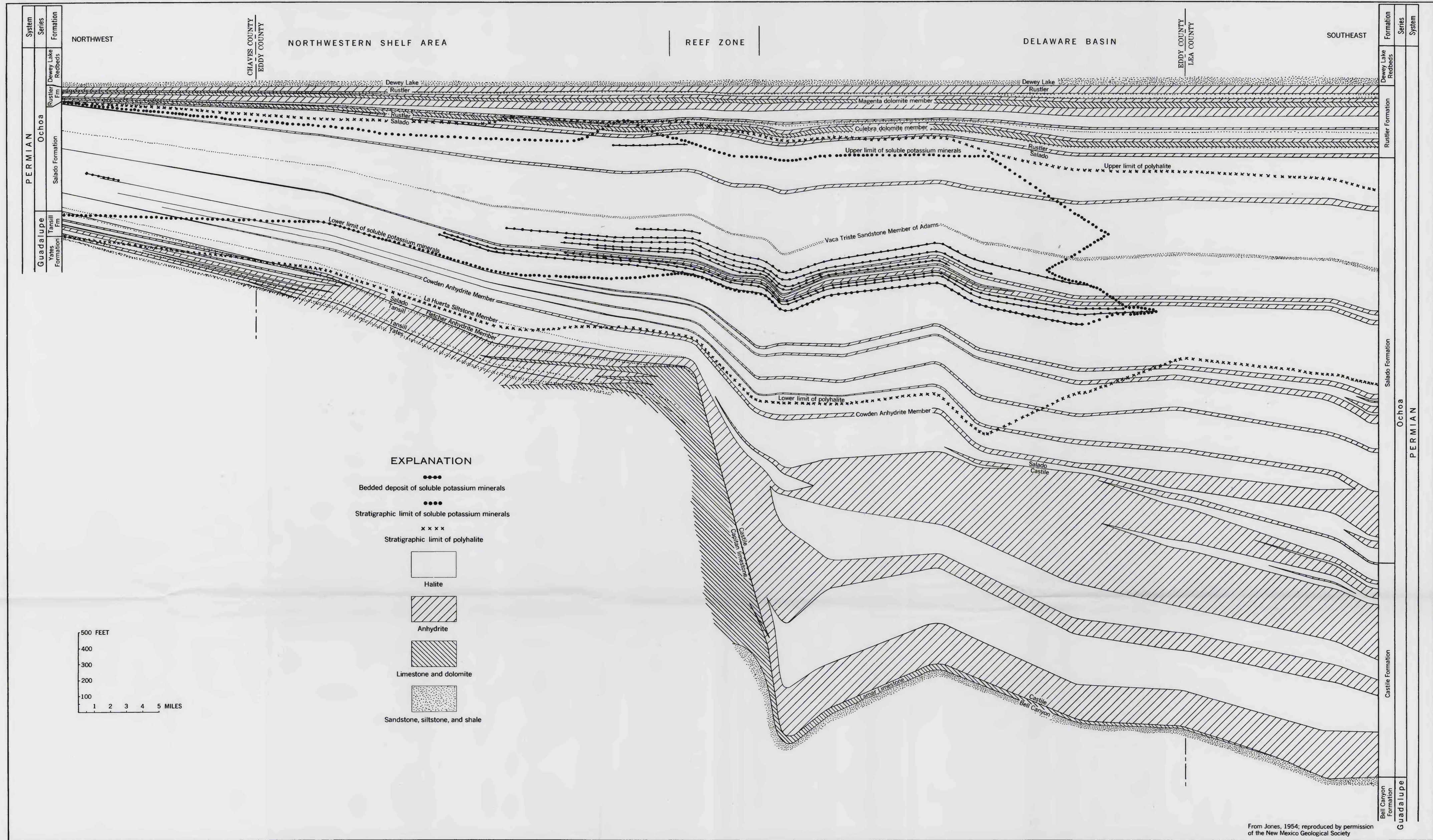
COMPOSITE CROSS SECTION SHOWING THE SUCCESSION OF EVAPORITES IN UPPER PERMIAN FORMATIONS, SOUTHEASTERN NEW MEXICO
