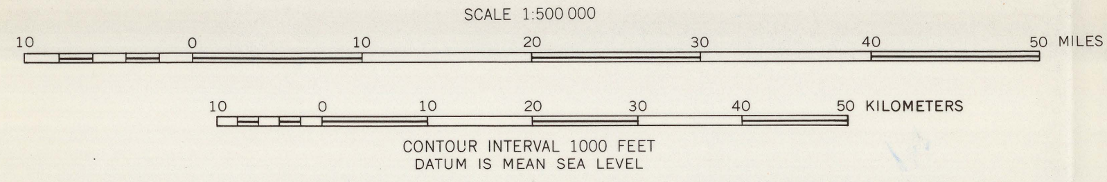
ISOHYETAL MAP OF UPPER COLORADO RIVER BASIN SHOWING AVERAGE MAY-SEPTEMBER PRECIPITATION
