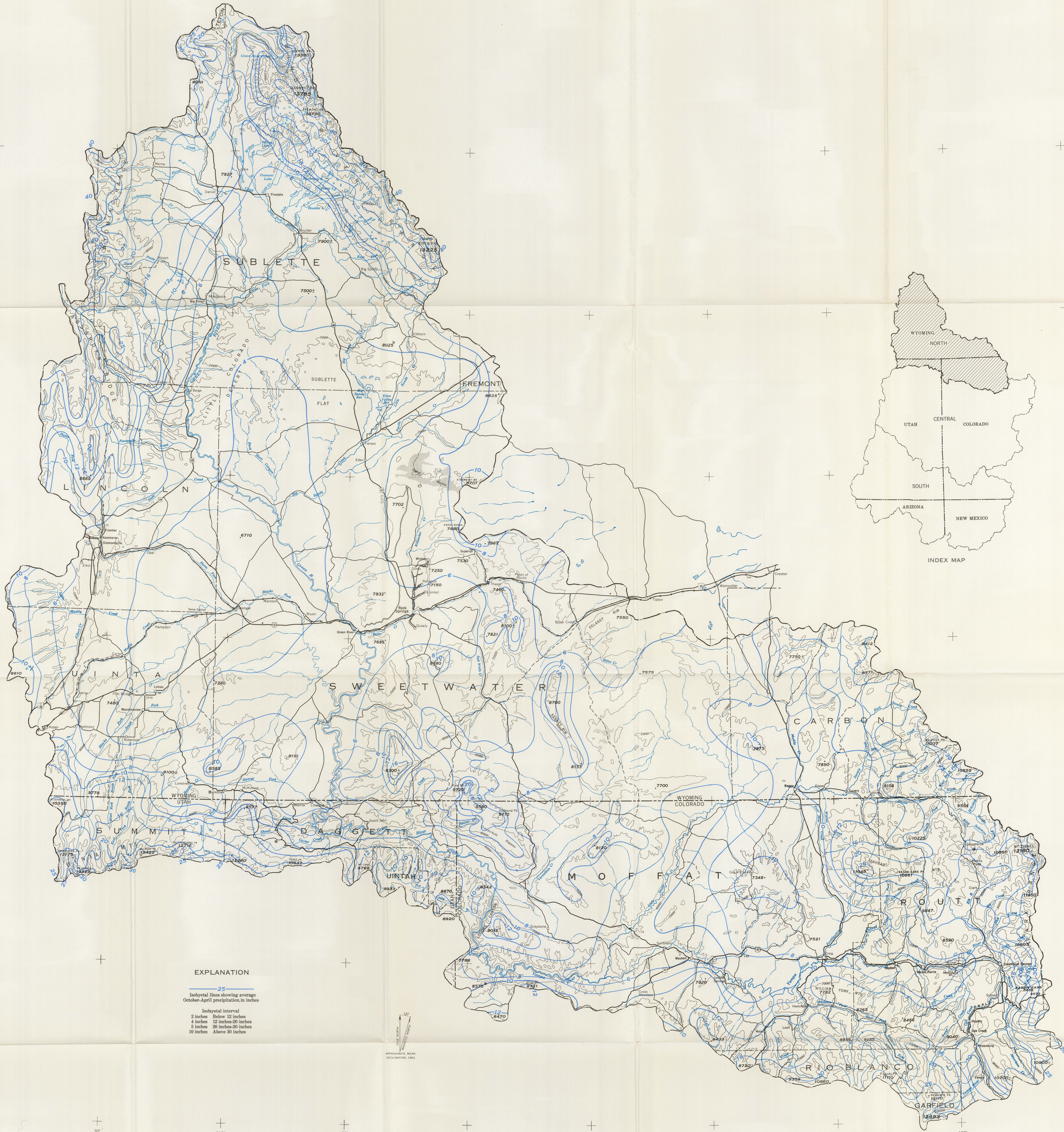
ISOHYETAL MAP OF UPPER COLORADO RIVER BASIN SHOWING AVERAGE OCTOBER-APRIL PRECIPITATION
