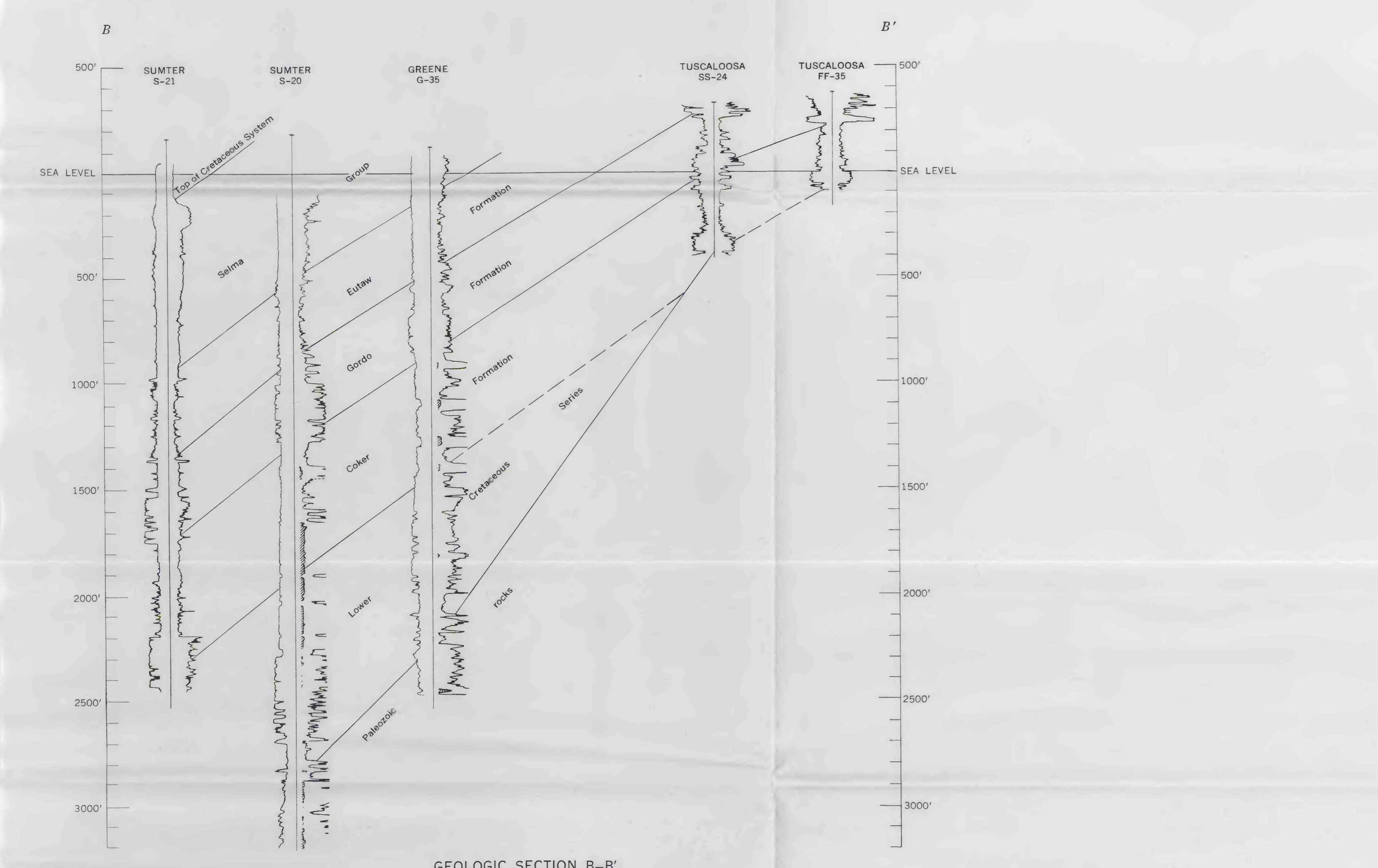
GEOLOGIC SECTION B-B'
