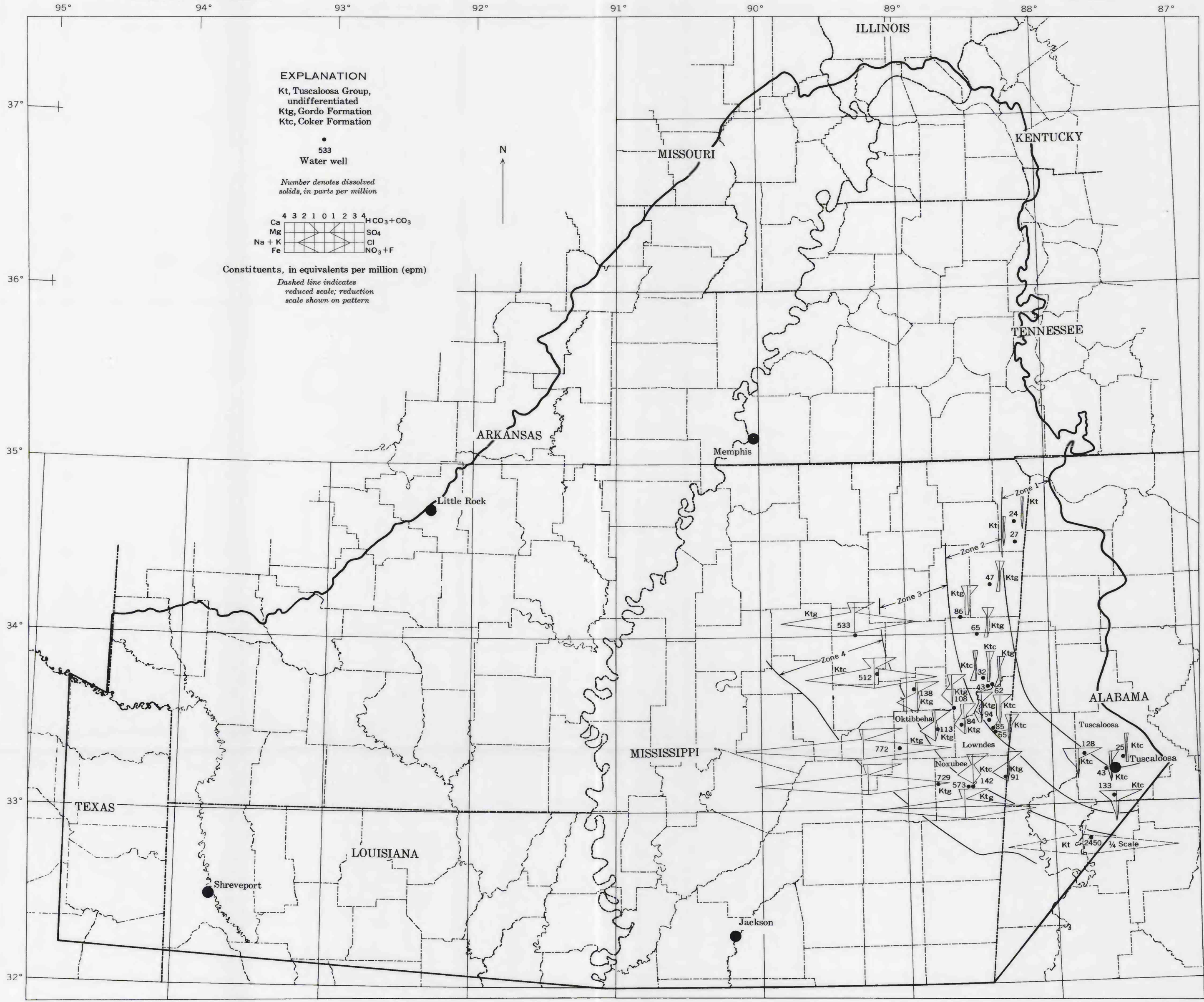
MAP SHOWING AREAL VARIATIONS IN THE CHEMICAL CHARACTERISTICS OF WATER FROM THE TUSCALOOSA GROUP IN THE MISSISSIPPI EMBAYMENT
