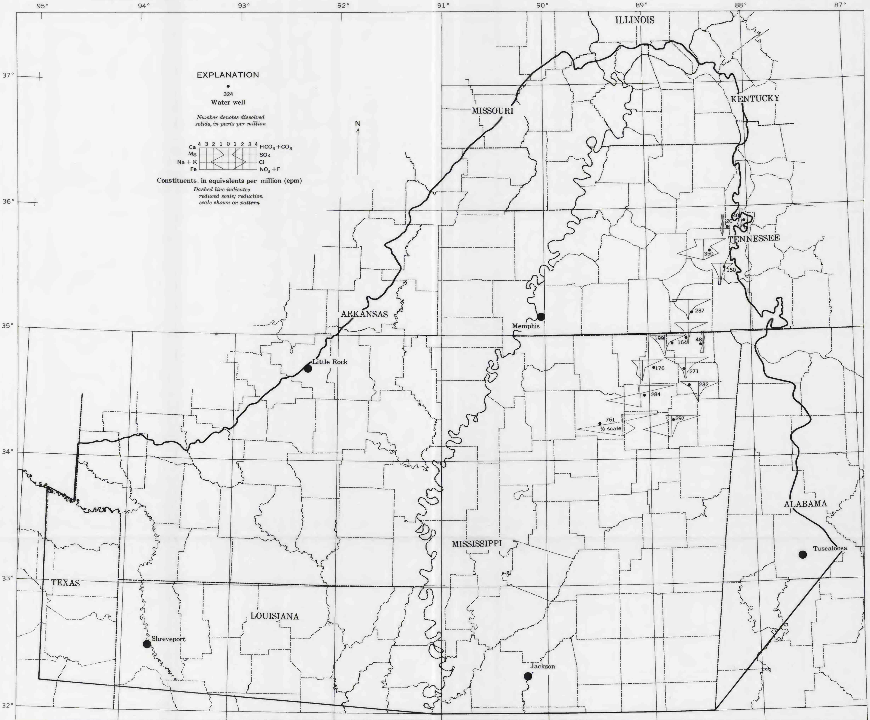
MAP SHOWING AREAL VARIATIONS IN THE CHEMICAL CHARACTERISTICS OF WATER FROM THE COFFEE SAND IN THE MISSISSIPPI EMBAYMENT
