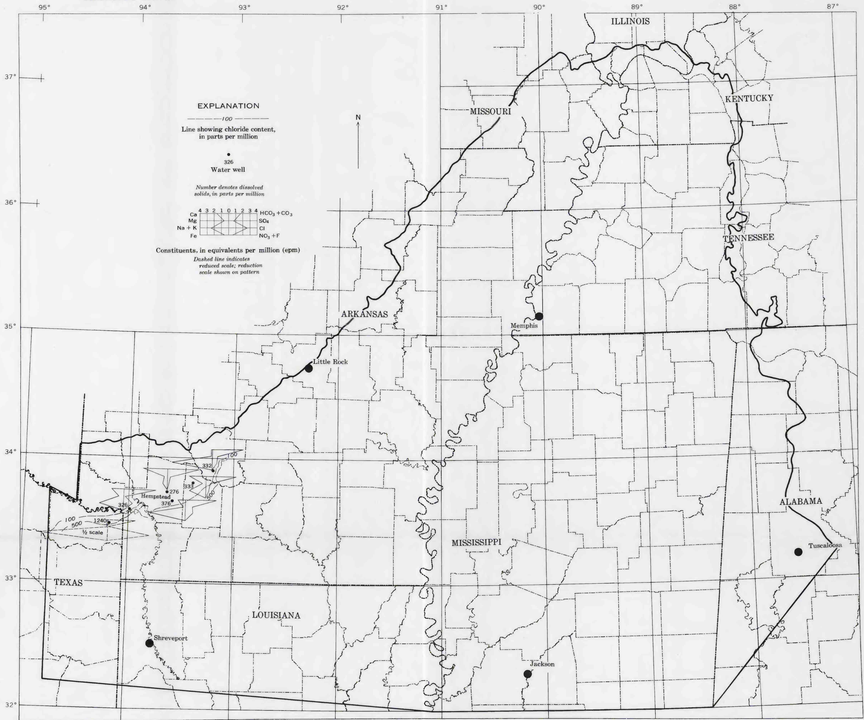
MAP SHOWING AREAL VARIATIONS IN THE CHEMICAL CHARACTERISTICS AND IN THE CHLORIDE CONTENT OF WATER FROM THE NACATOCH SAND IN THE MISSISSIPPI EMBAYMENT
