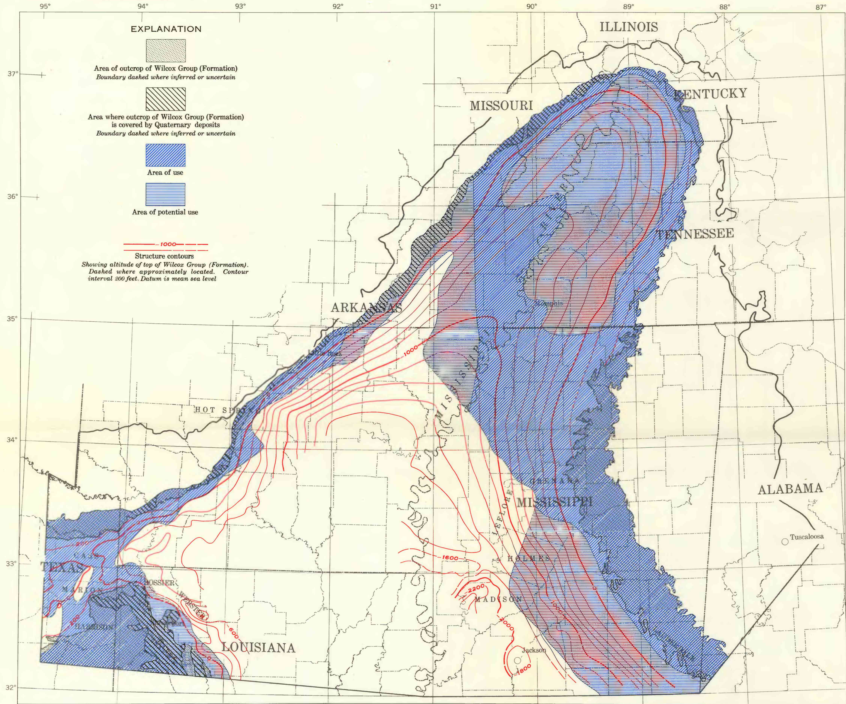
TOP OF UNIT AND AREAS OF WATER USE
