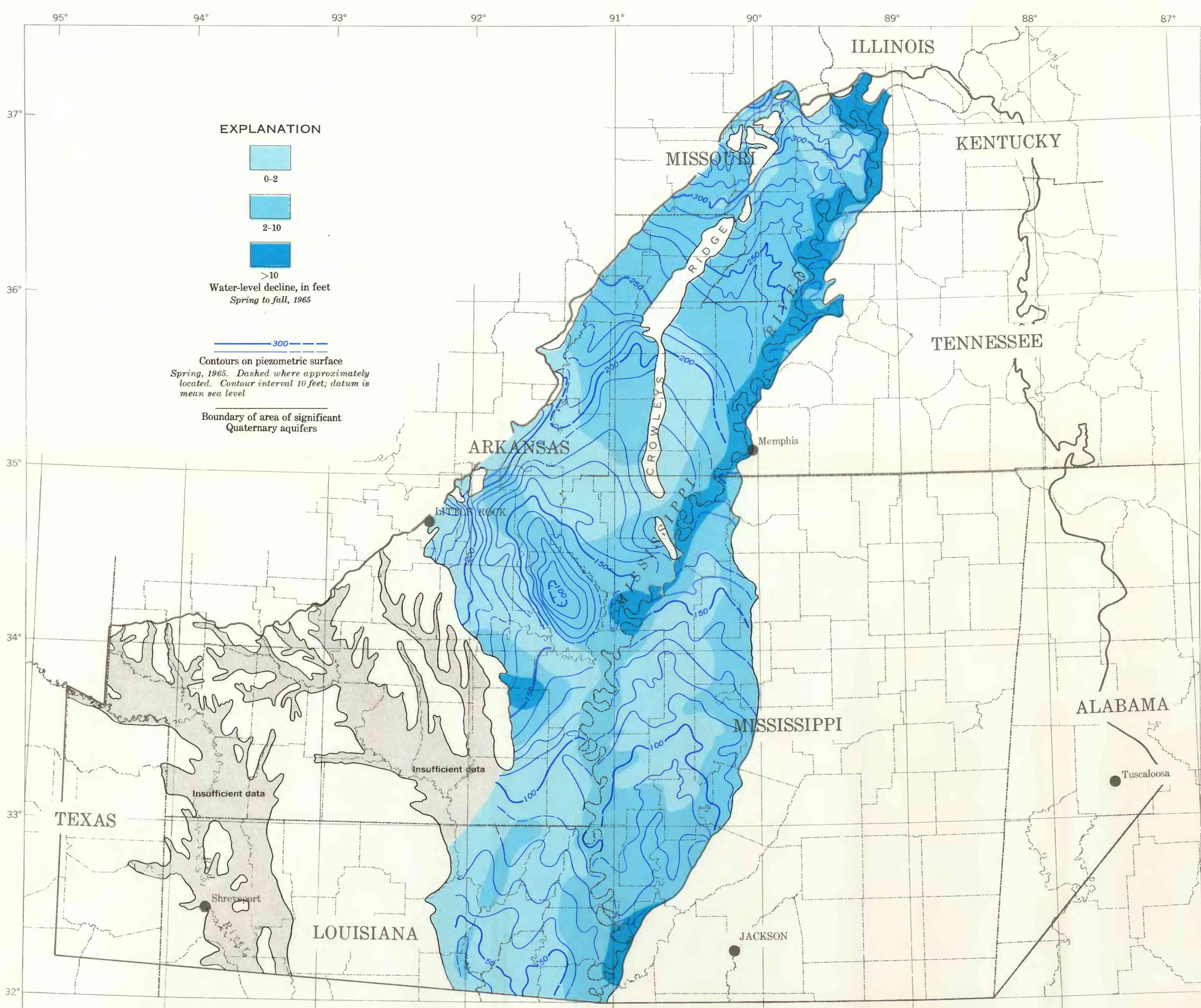
PIEZOMETRIC SURFACE AND WATER-LEVEL DECLINE, 1965
