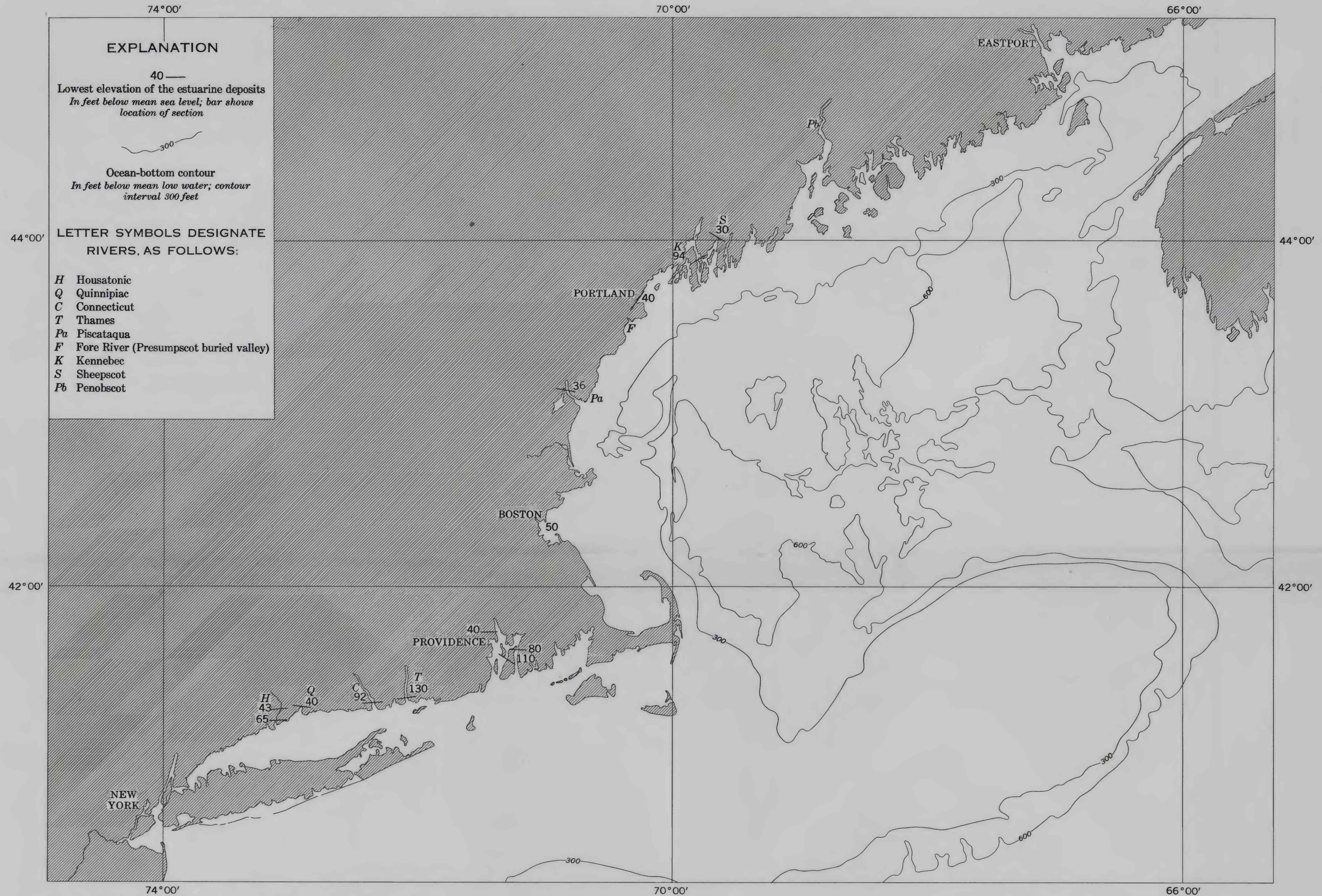
MAP OF THE NEW ENGLAND COAST SHOWING ELEVATIONS OF THE THALWEGS OF PRE-ESTUARINE VALLEYS
