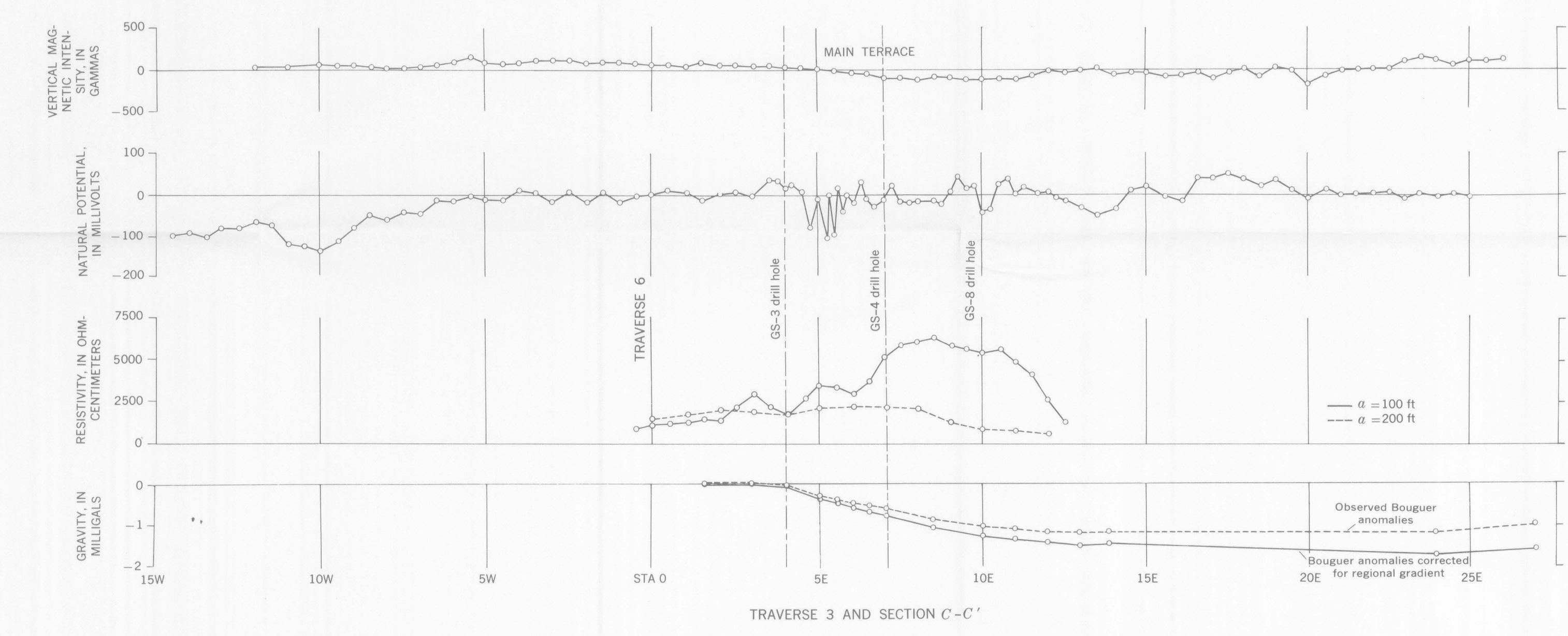
GEOPHYSICAL DATA FROM SELECTED TRAVERSES, NORTHERN PART OF THE STEAMBOAT SPRINGS THERMAL AREA, WASHOE COUNTY, NEVADA
