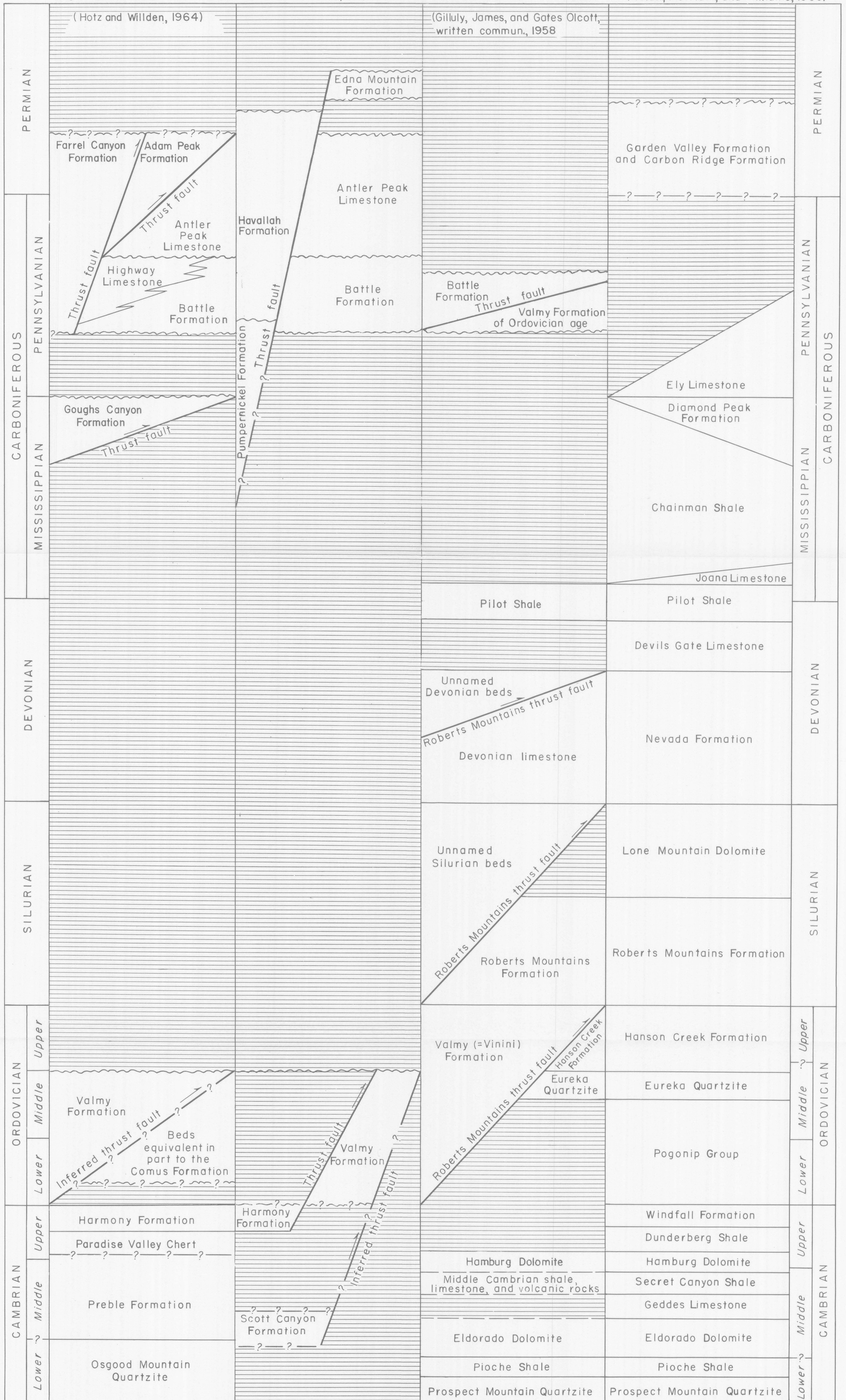
CORRELATION CHART OF PALEOZOIC FORMATIONS, NORTH CENTRAL NEVADA
