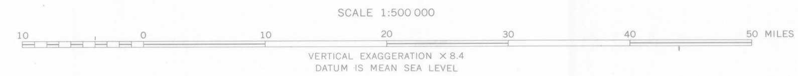
SCHEMATIC STRUCTURE SECTIONS ACROSS THE SOUTHWESTERN PART OF THE WILLISTON BASIN, MONTANA, NORTH AND SOUTH DAKOTA
