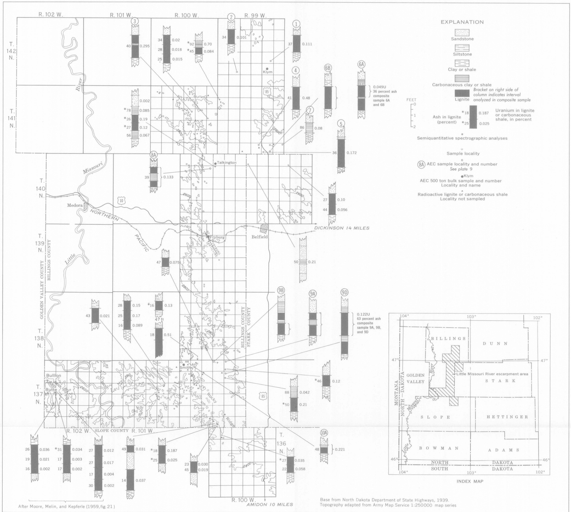
MAP SHOWING LOCATIONS OF SELECTED URANIUM OCCURRENCES LITTLE MISSOURI RIVER ESCARPMENT AREA, NORTH DAKOTA
