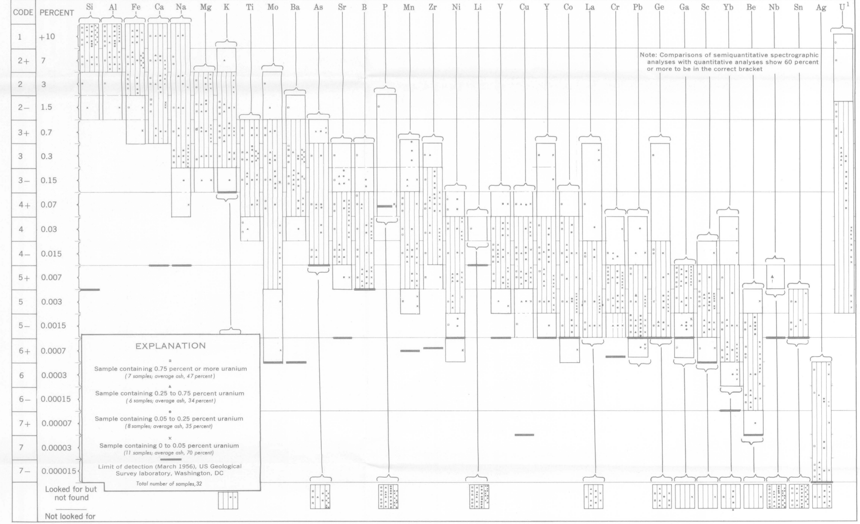
E. RADIOACTIVE LIGNITE AND CARBONACEOUS SHALE ASH FROM SENTINEL BUTTE MEMBER OF FORT UNION FORMATION, LITTLE MISSOURI RIVER ESCARPMENT SOUTHWESTERN NORTH DAKOTA
