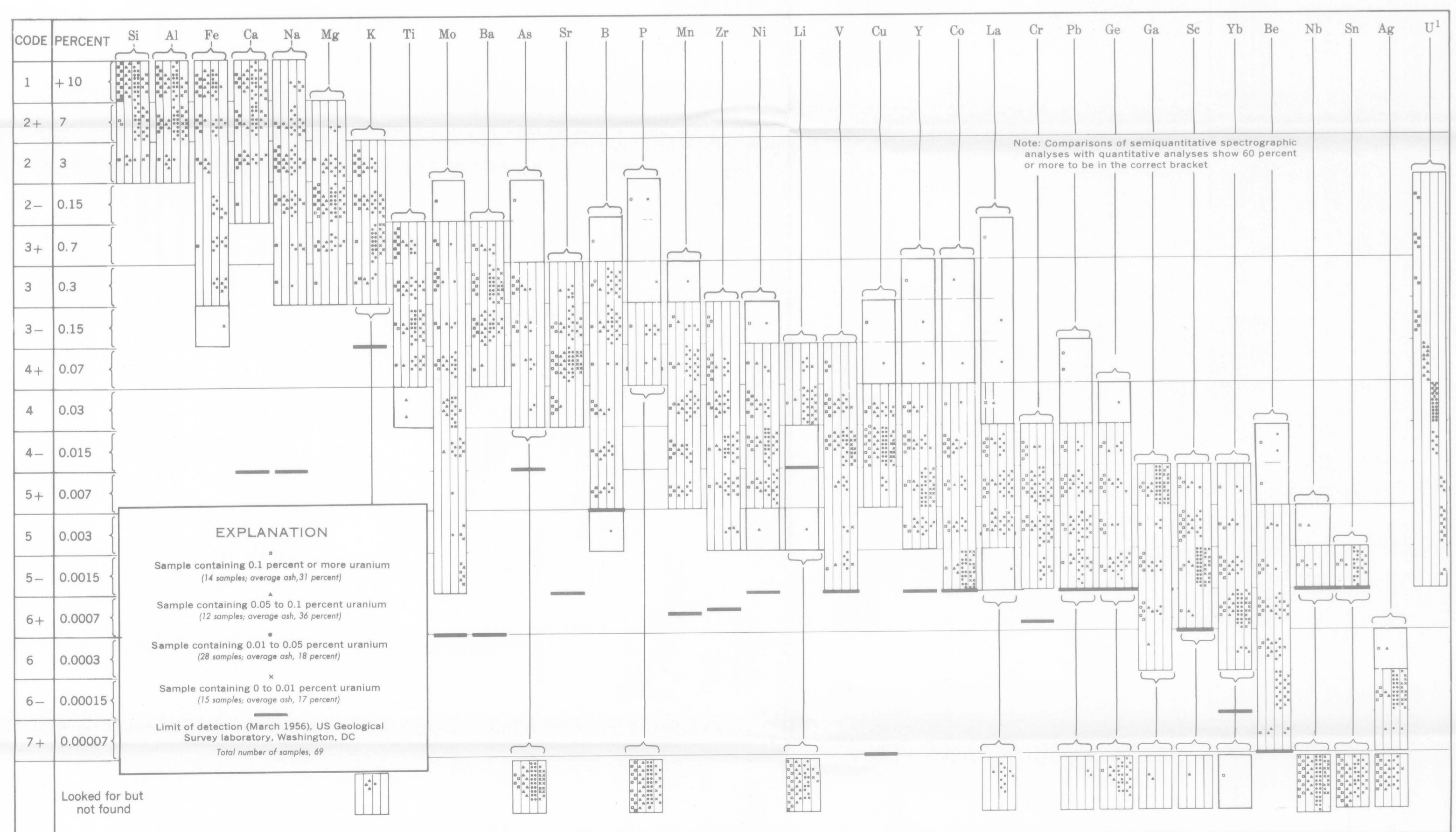
C. RADIOACTIVE LIGNITE AND CARBONACEOUS SHALE ASH FROM LUDLOW MEMBER OF FORT UNION FORMATION, SLIM BUTTES, HARDING COUNTY, SOUTH DAKOTA
