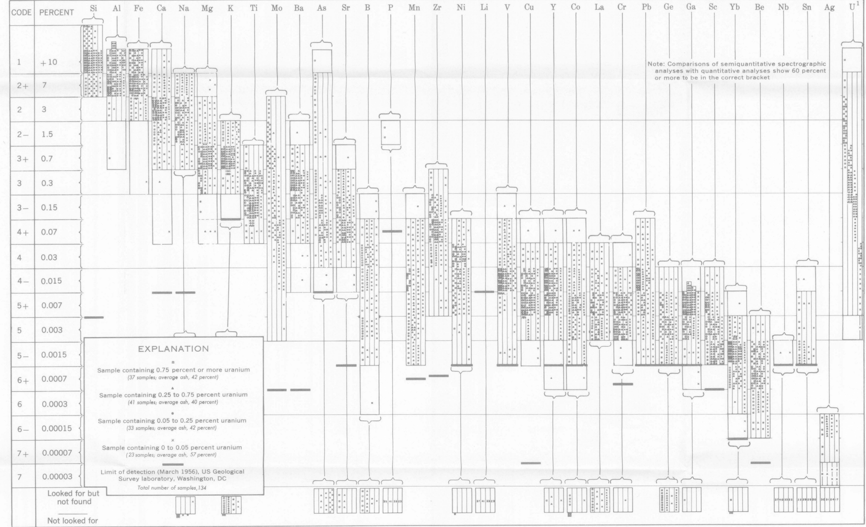
D. RADIOACTIVE LIGNITE AND CARBONACEOUS SHALE ASH FROM TONGUE RIVER MEMBER OF FORT UNION FORMATION, NORTH CAVE HILLS, SOUTH DAKOTA
