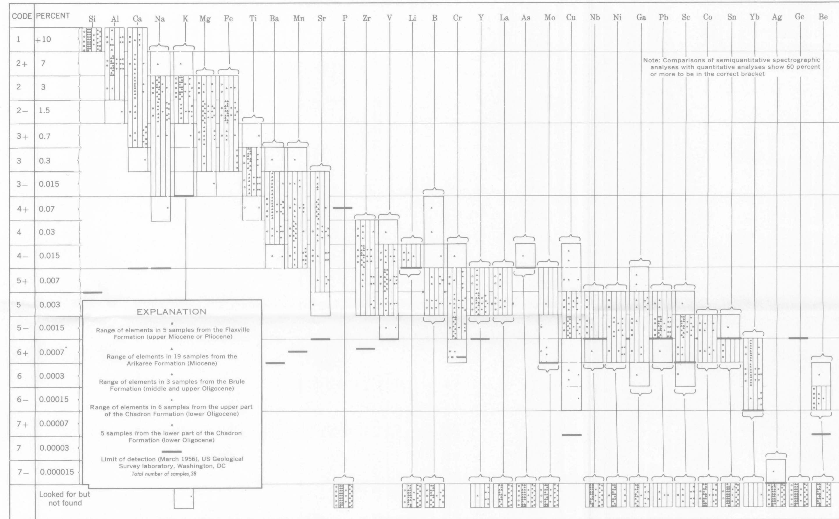
A. REPRESENTATIVE ROCK SAMPLES FROM THE CHADRON, BRULE, ARIKAREE, AND FLAXVILLE FORMATIONS, EASTERN MONTANA, NORTH AND SOUTH DAKOTA
