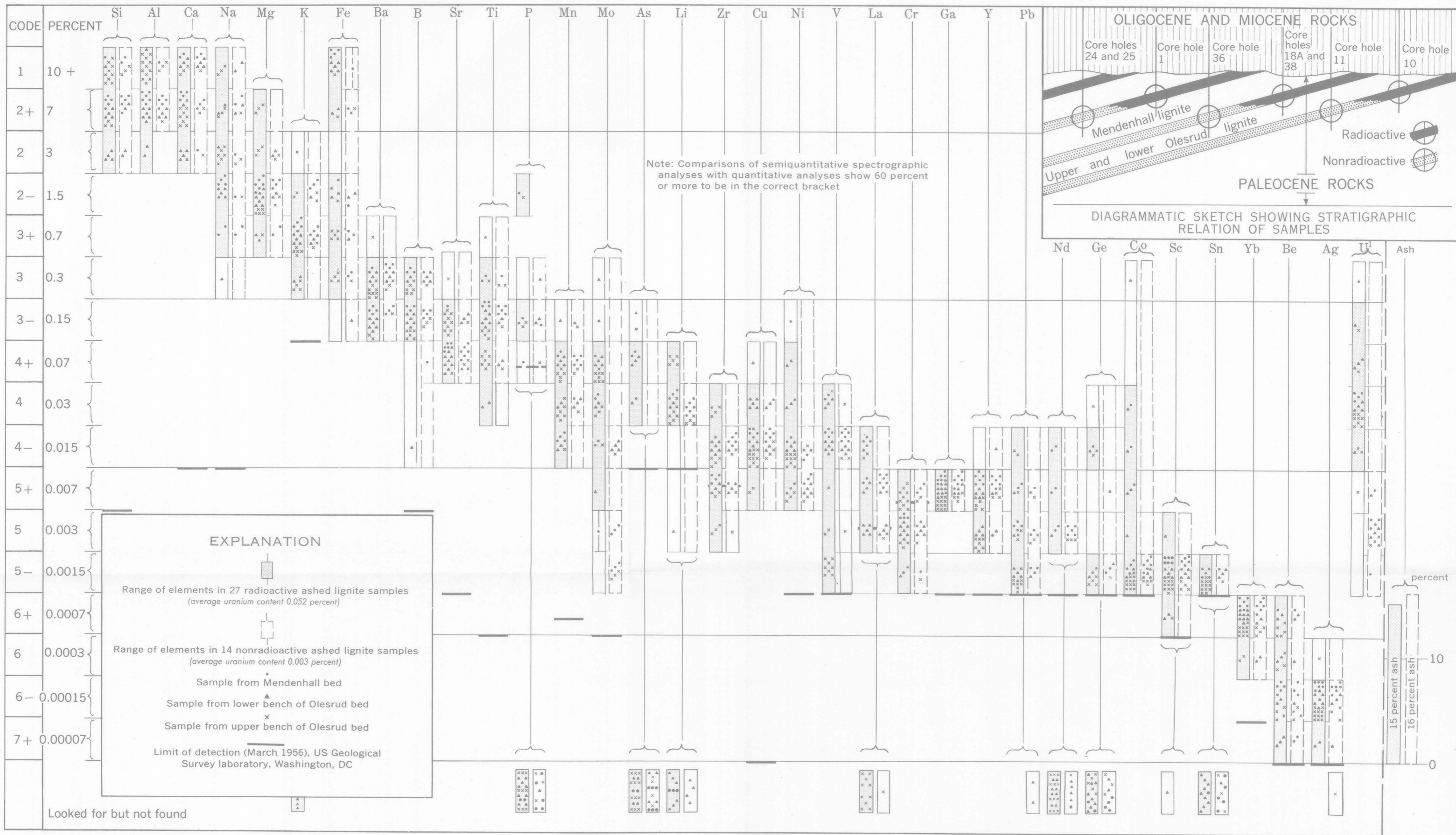
COMPARISON OF DATA FROM SEMIQUANTITATIVE SPECTROGRAPHIC ANALYSES OF RADIOACTIVE AND NONRADIOACTIVE LIGNITE CORE FROM SLIM BUTTES, HARDING COUNTY, SOUTH DAKOTA
