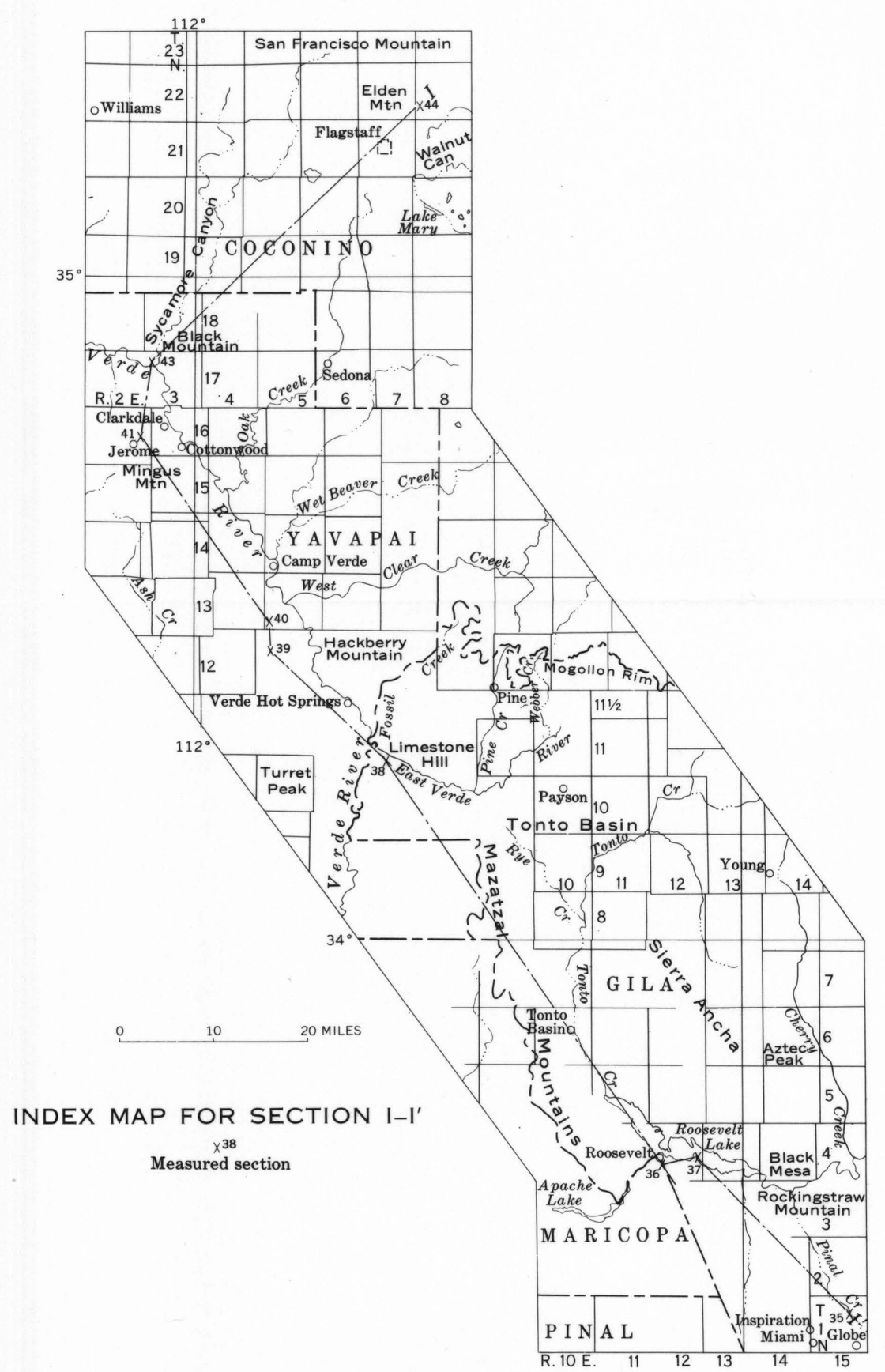
SECTION I-I', BECKERS BUTTE AND JEROME MEMBERS OF THE MARTIN FORMATION, CENTRAL ARIZONA
