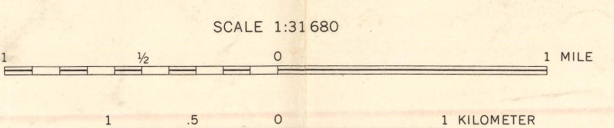
GEOLOGIC MAP OF THE MOUNT LEWIS AND CRESCENT VALLEY QUADRANGLES, NEVADA
