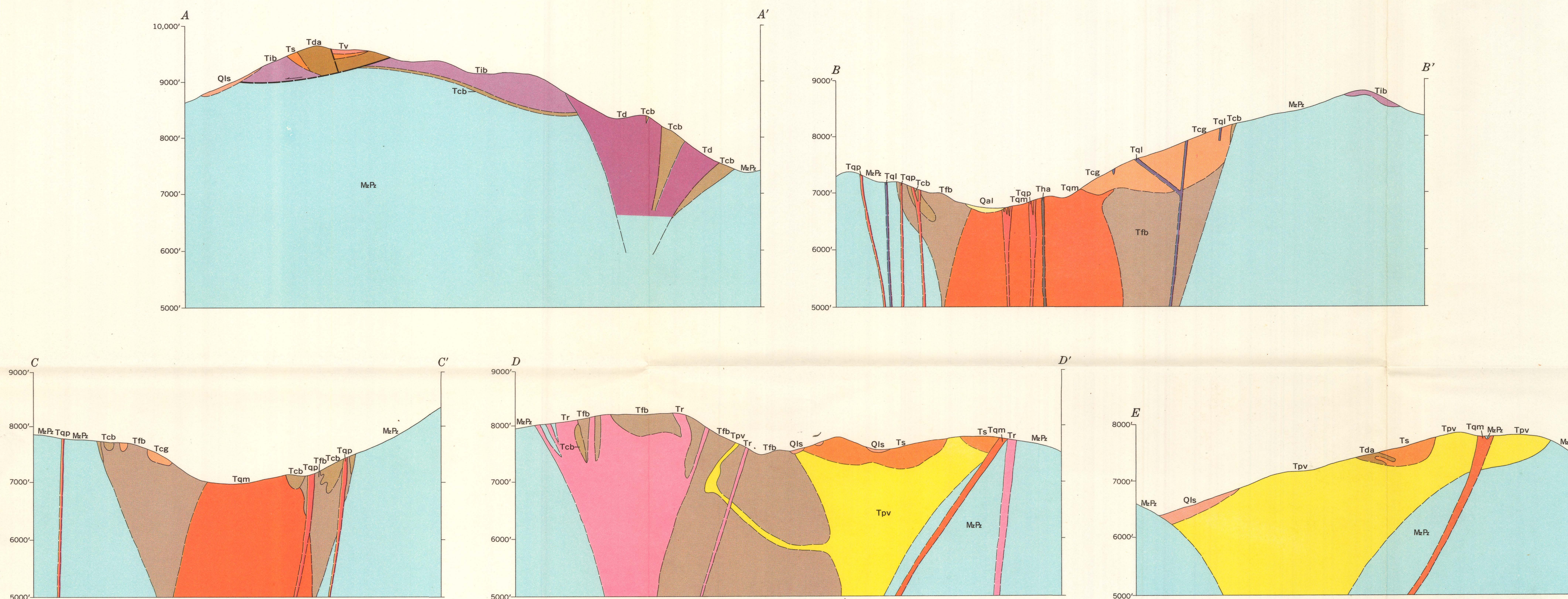
GEOLOGIC MAP AND SECTIONS OF THE BRECCIA PIPES OF THE MOUNT LEWIS QUADRANGLE, NEVADA
