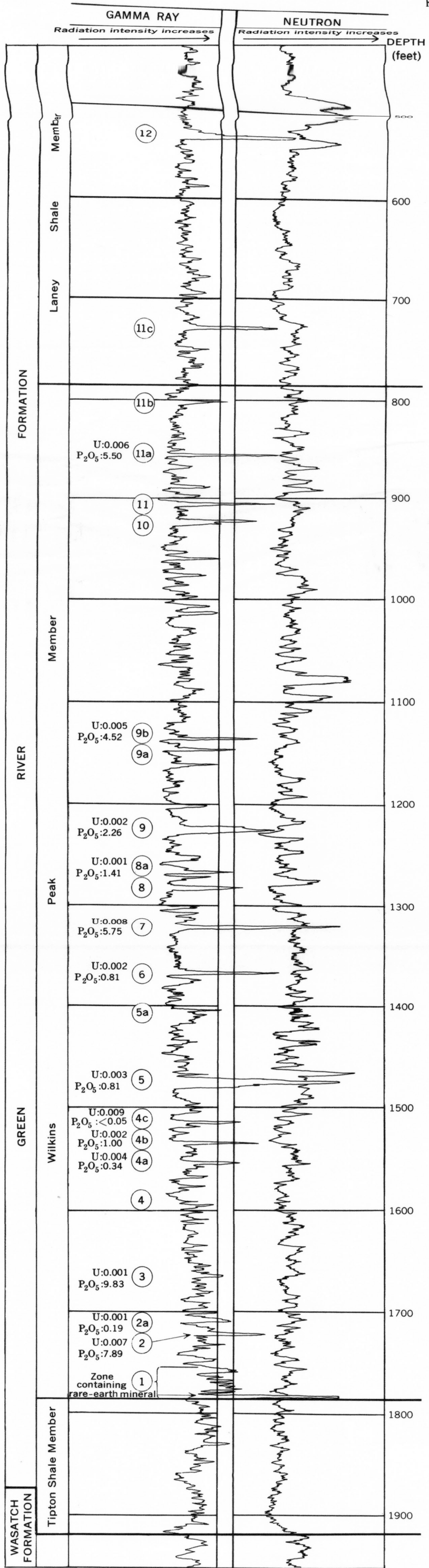
GAMMA RAY-NEUTRON LOG OF PERKINS, GREEN RIVER 3 CORE HOLE SEC. 8, T. 17 N., R. 107 W., WYOMING, SHOWING LOG CHARACTERISTICS OF WILKINS PEAK MEMBER OF THE GREEN RIVER FORMATION AND POSITIONS OF URANIFEROUS PHOSPHATIC ZONES (CORE ANALYSES ARE IN PERCENT.)
