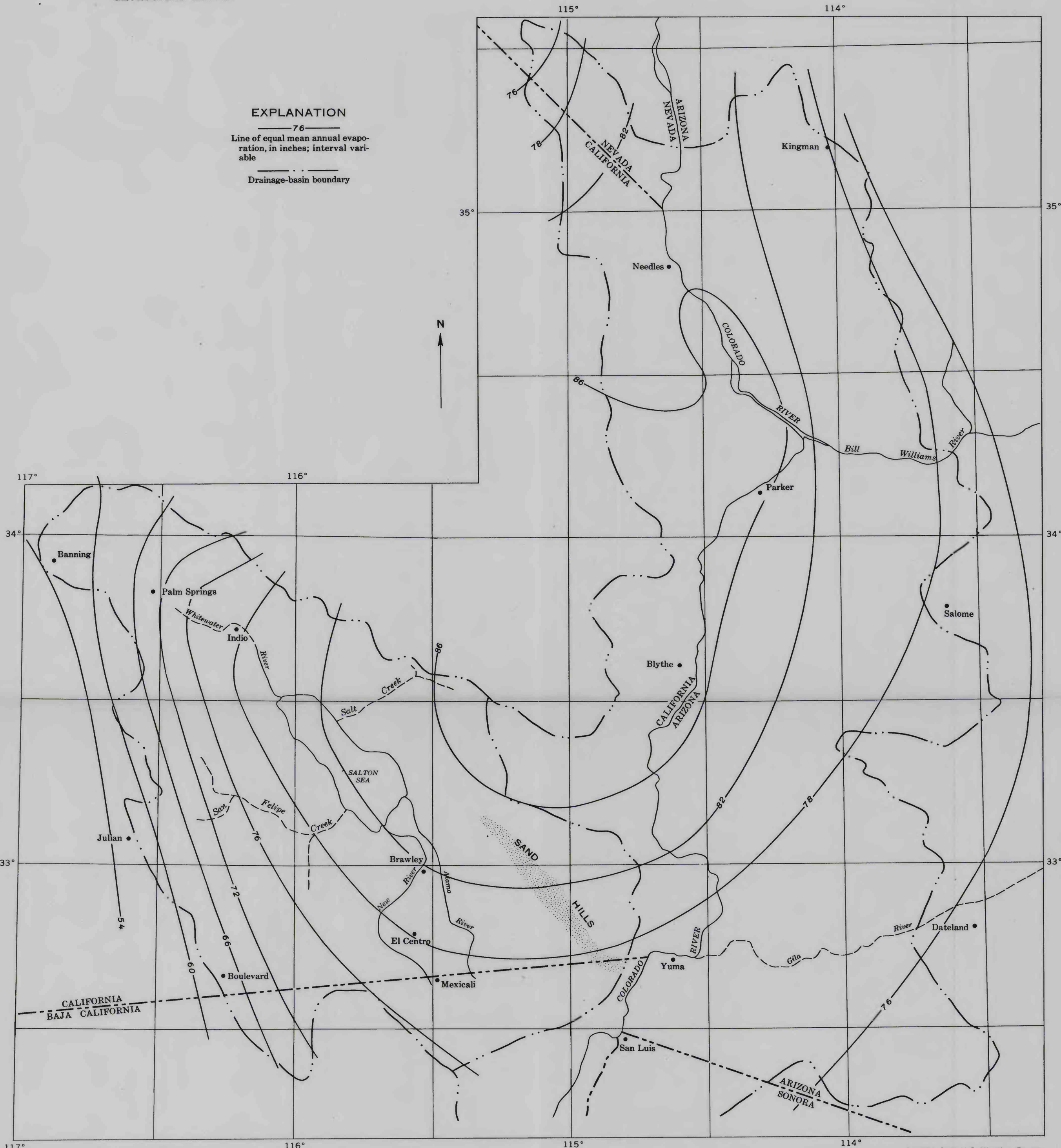
MAP SHOWING MEAN ANNUAL LAKE EVAPORATION, 1946-55 LOWER COLORADO RIVER-SALTON SEA AREA
