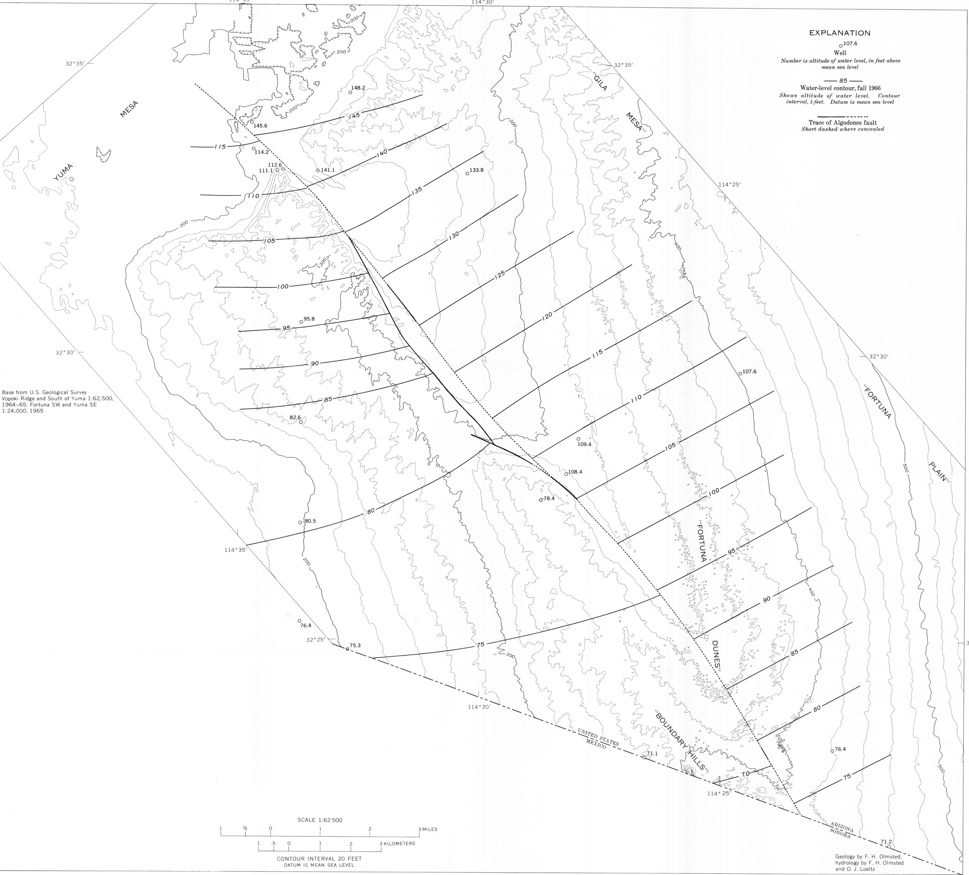
TOPOGRAPHIC MAP OF THE "UPPER MESA" SHOWING TRACE OF THE ALGODONES FAULT AND THE EFFECT OF THE FAULT ON GROUND-WATER LEVELS, YUMA AREA, ARIZONA AND CALIFORNIA
