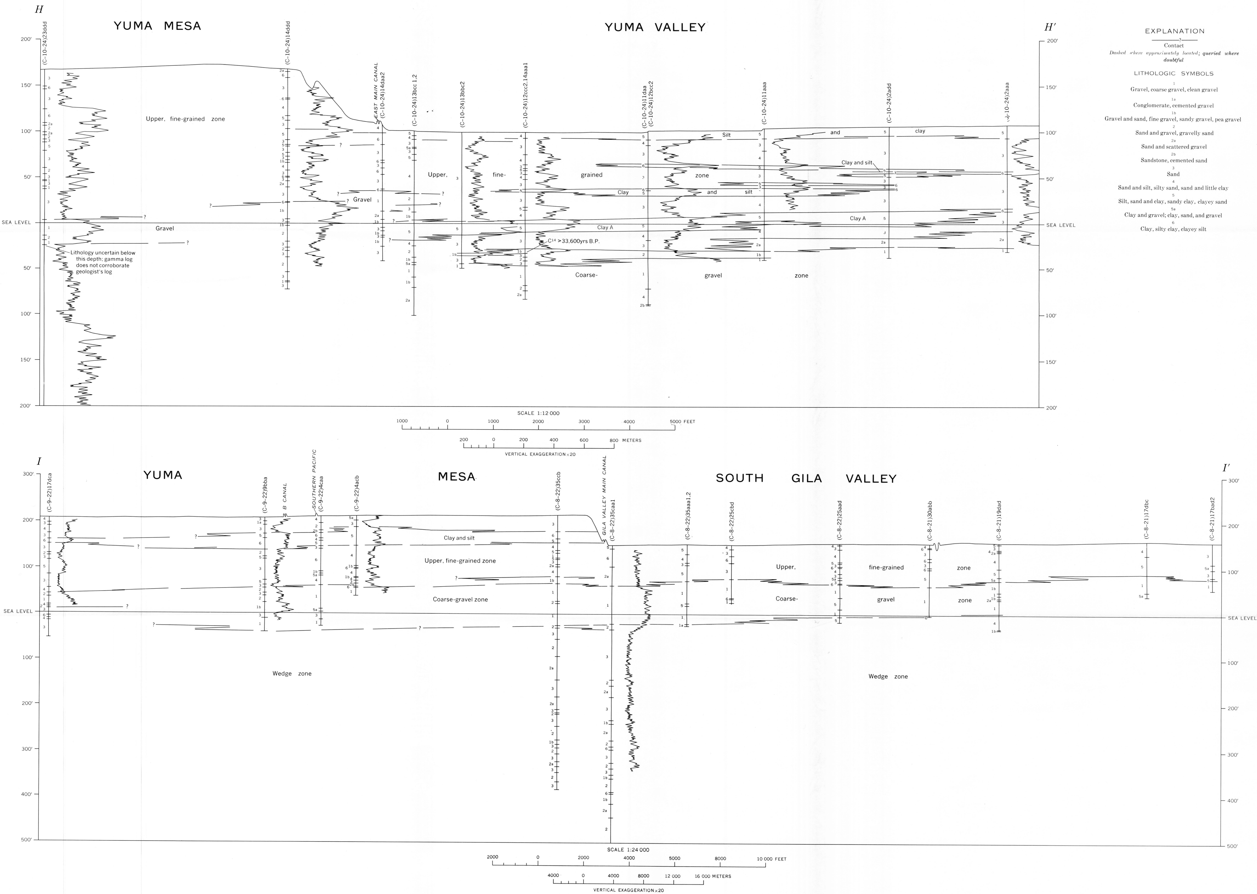
GEOLOGIC SECTIONS H-H' ACROSS MARGINS OF YUMA VALLEY AND YUMA MESA SOUTHEAST OF SOMERTON AND I-I' ACROSS EASTERN SOUTH GILA VALLEY AND NORTHEASTERN YUMA MESA, YUMA AREA, ARIZONA AND CALIFORNIA
