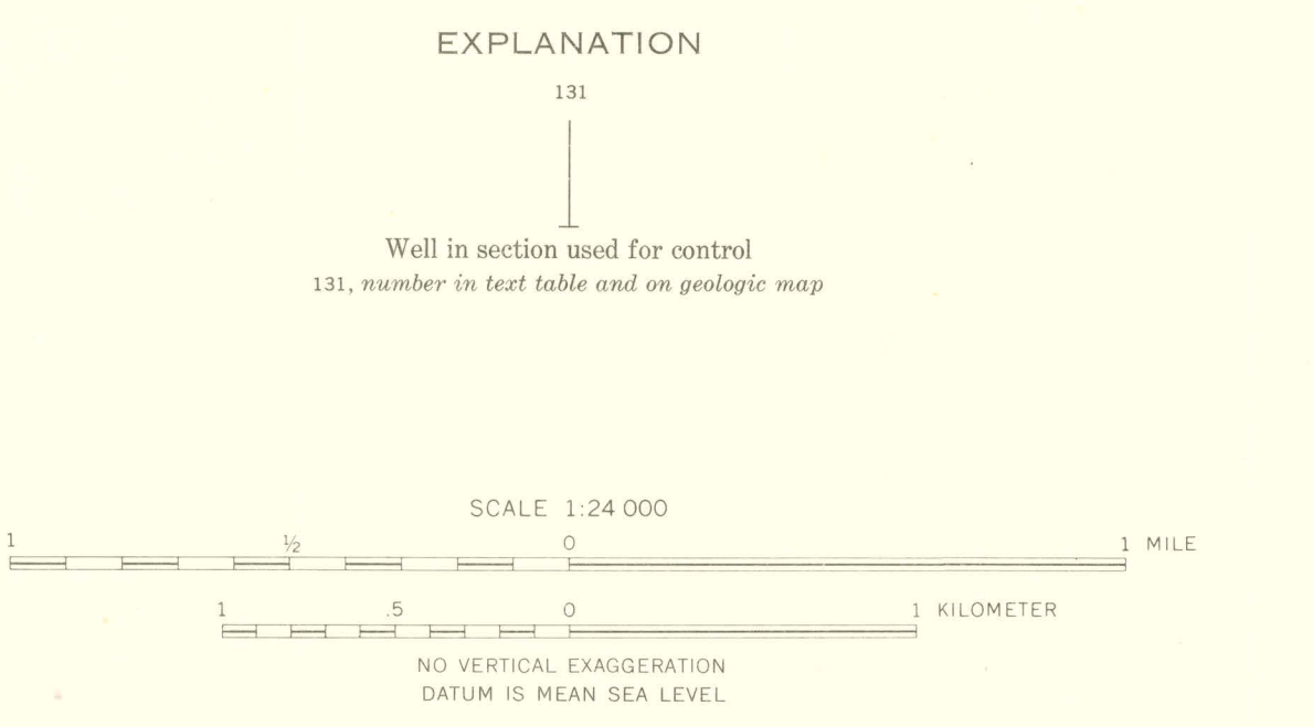
STRATIGRAPHIC AND STRUCTURE SECTIONS, E-E' to N-N', IN THE GRANITE MOUNTAINS AREA, CENTRAL WYOMING Lines of sections shown on plate 1
