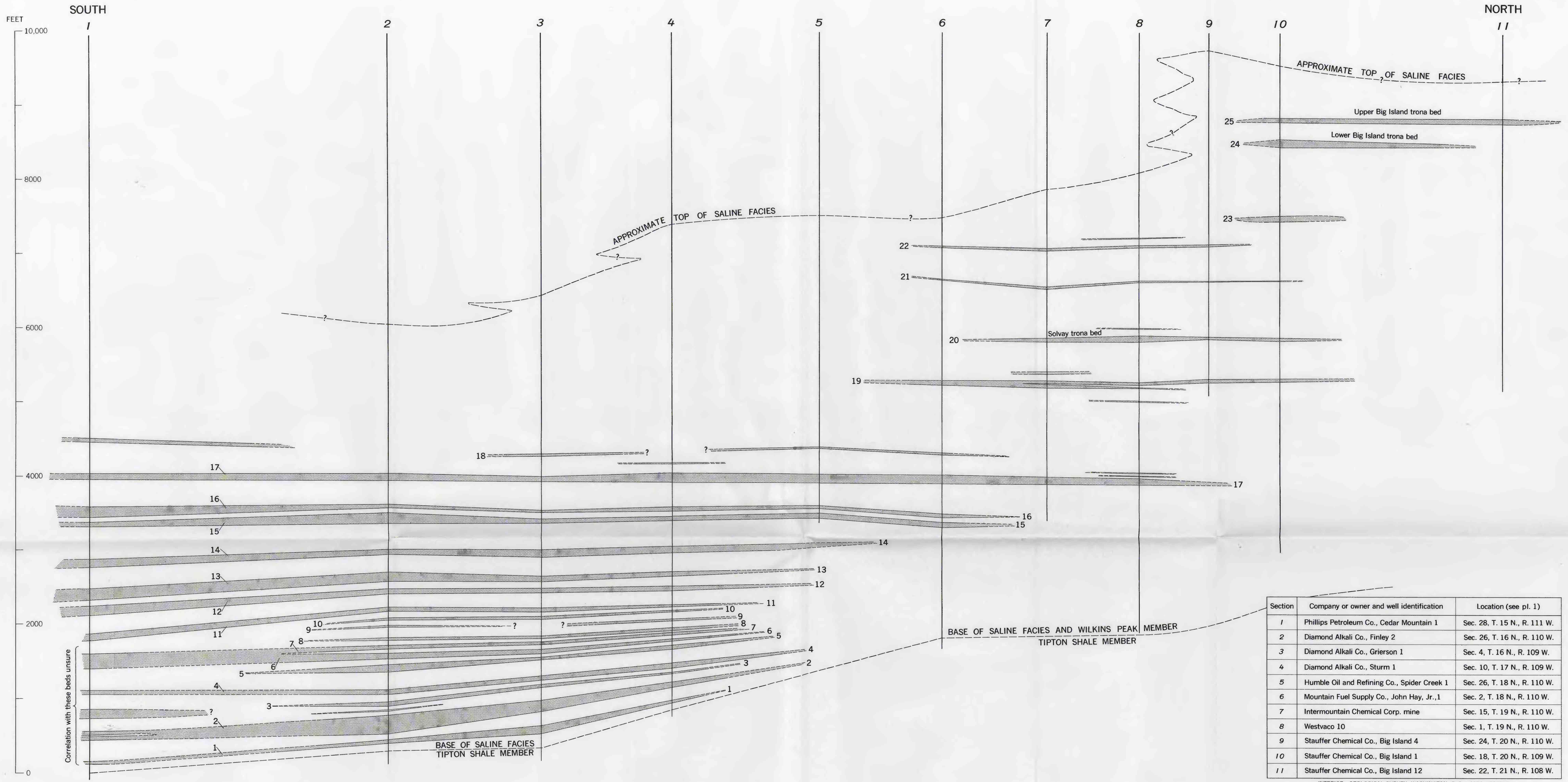
NORTH-SOUTH SECTION OF A PART OF THE WILKINS PEAK MEMBER SHOWING THE EXTENT AND STRATIGRAPHIC RELATIONS OF THE TRONA AND TRONA-HALITE BEDS IN THE GREEN RIVER BASIN
