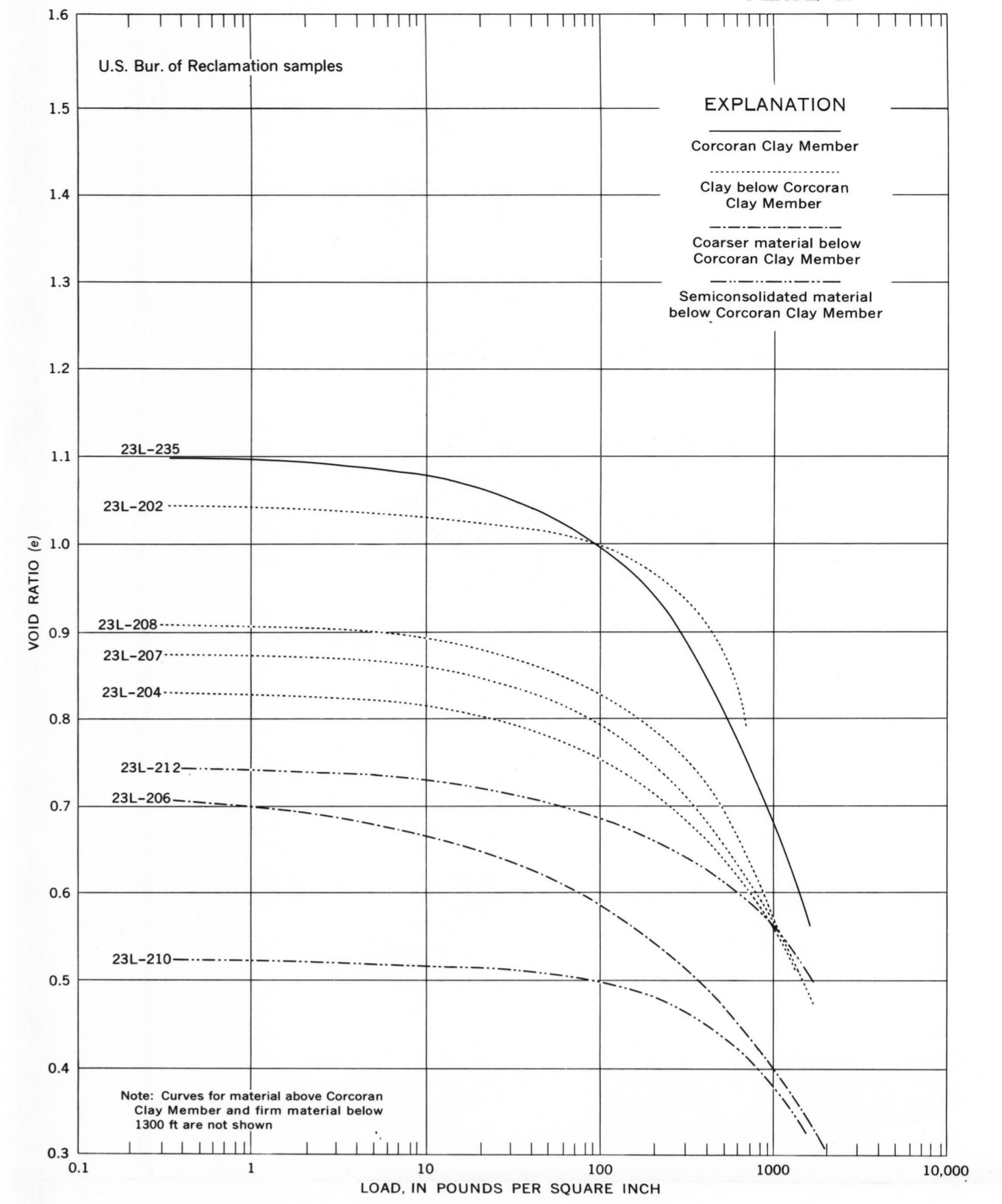
C. CORE HOLE 16/15-34N1, LOS BANOS-KETTLEMAN CITY AREA
