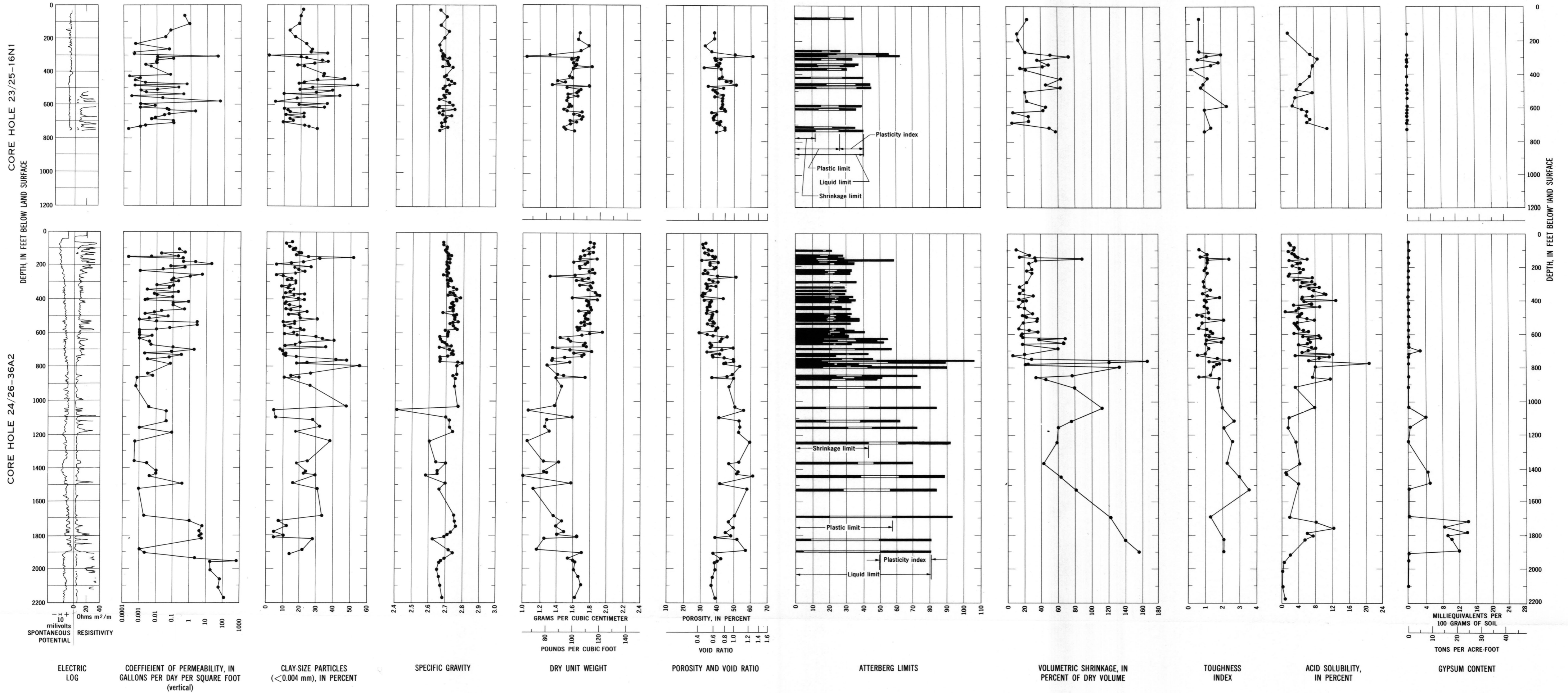
GRAPHS OF PHYSICAL PROPERTIES OF SAMPLES FROM CORE HOLES IN THE TULARE-WASCO AREA, CENTRAL CALIFORNIA
