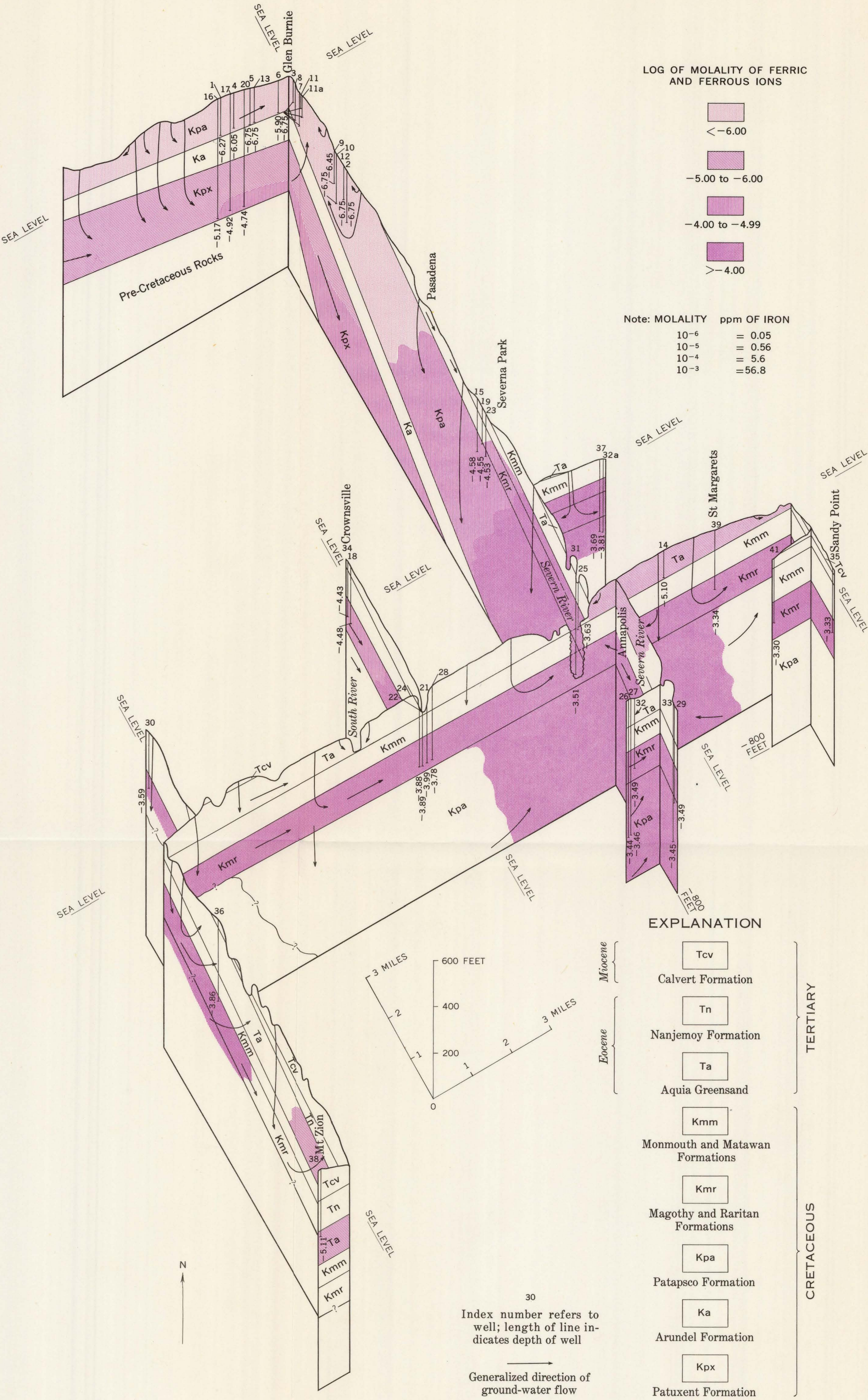
FENCE DIAGRAM SHOWING DISTRIBUTION OF THE MOLALITY OF THE FERRIC AND FERROUS IONS, ANNE ARUNDEL COUNTY, MARYLAND
