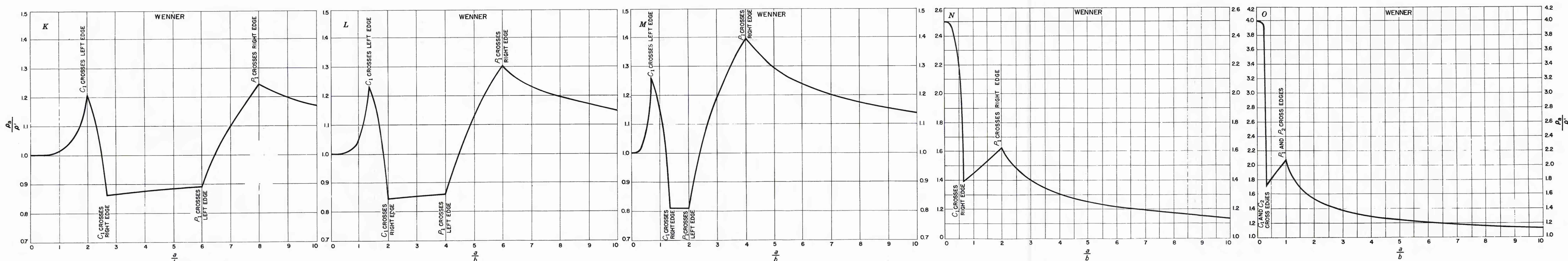
VERTICAL RESISTIVITY PROFILES ACROSS A VERTICAL DIKE OF UNIT WIDTH b , AND \rho''=4\rho' FOR ALL CURVES Lee and Wenner configurations. Center of configuration taken at various distances from dike
