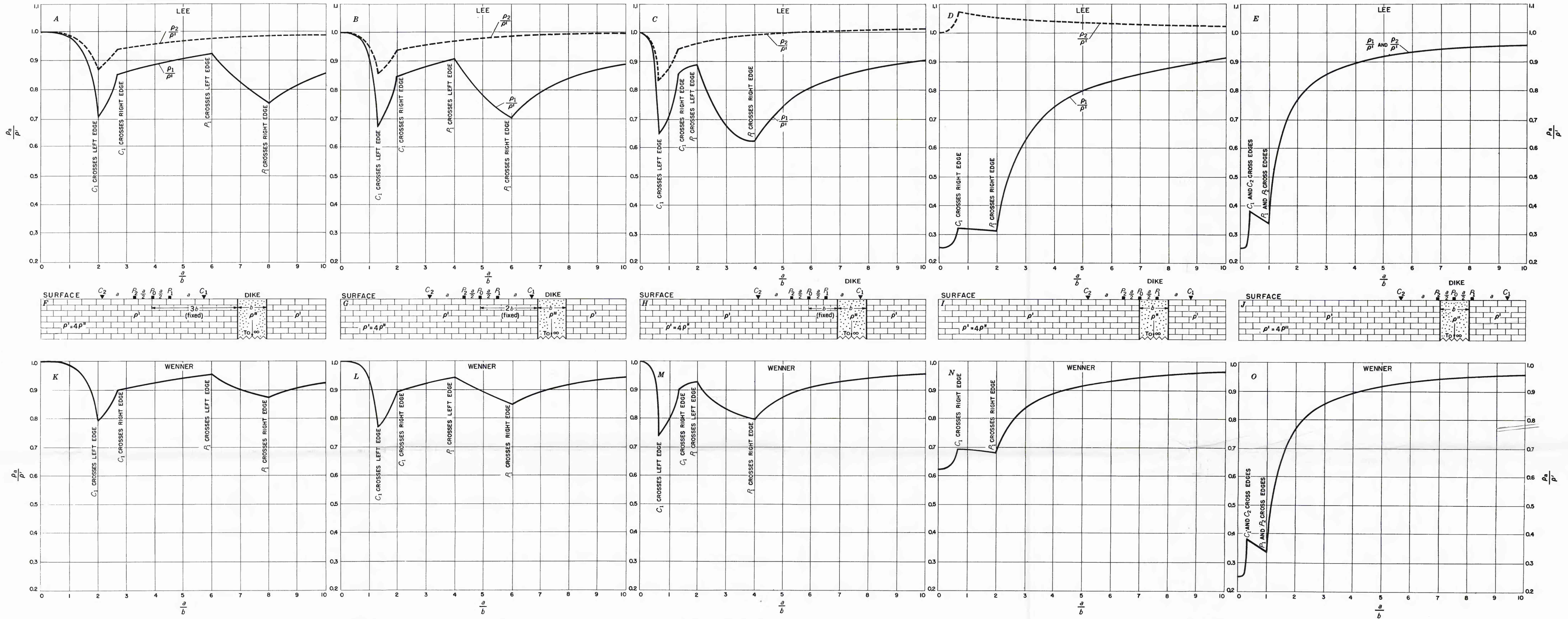
VERTICAL RESISTIVITY PROFILES ACROSS A VERTICAL DIKE OF UNIT WIDTH b , AND \rho'' = \frac{\rho'}{4} FOR ALL CURVES Lee and Wenner configurations. Center of configuration taken at various distances from dike
