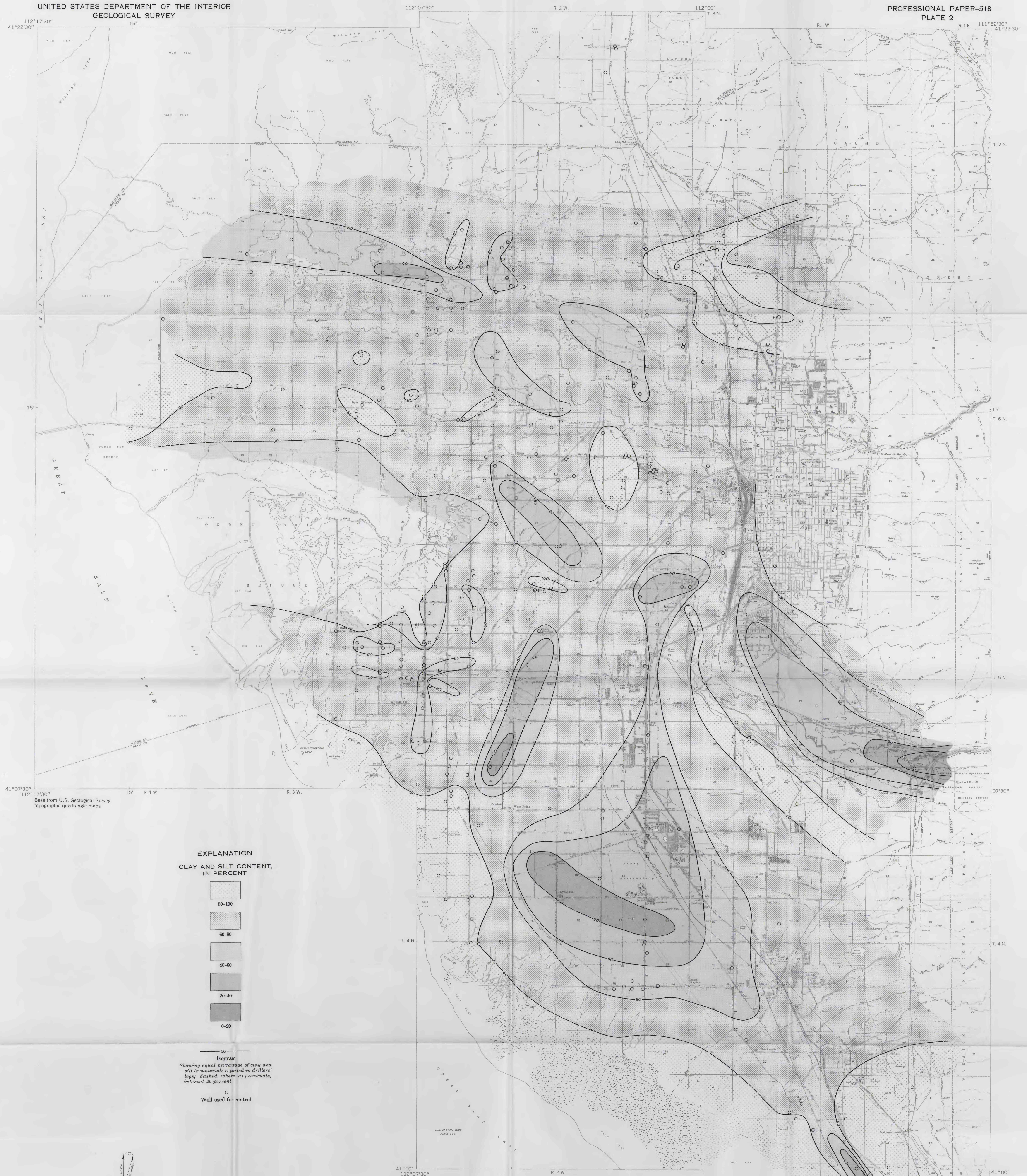
MAP OF THE WEBER DELTA DISTRICT, UTAH, SHOWING THE RATIO, IN PERCENT, OF CLAY AND SILT IN THE MATERIALS REPORTED IN DRILLERS' LOGS FOR THE SECTION BETWEEN THE LAND SURFACE AND A DEPTH OF 200 FEET
