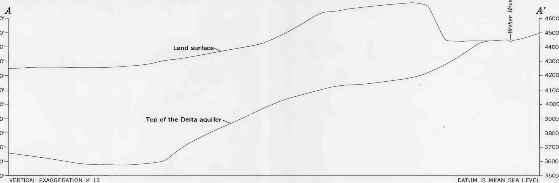
CONTOUR MAP AND PROFILE OF TOP OF DELTA AQUIFER, WEBER DELTA DISTRICT, UTAH
