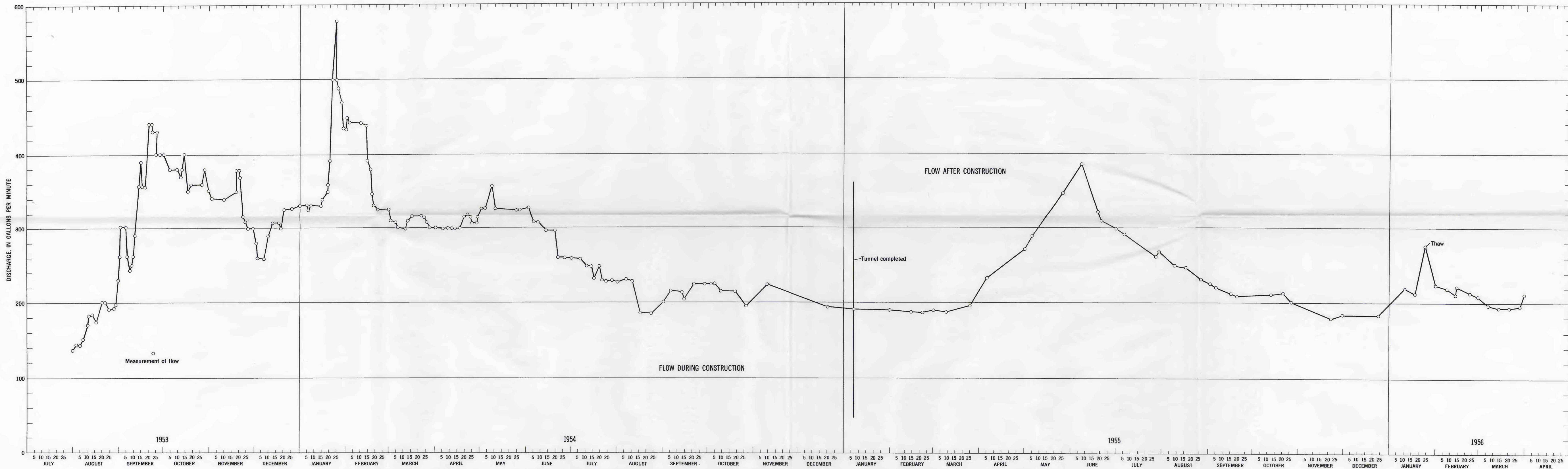
HYDROGRAPH OF DISCHARGE FROM GATEWAY TUNNEL, JULY 1953 TO MARCH 1956, WEBER DELTA DISTRICT, UTAH
