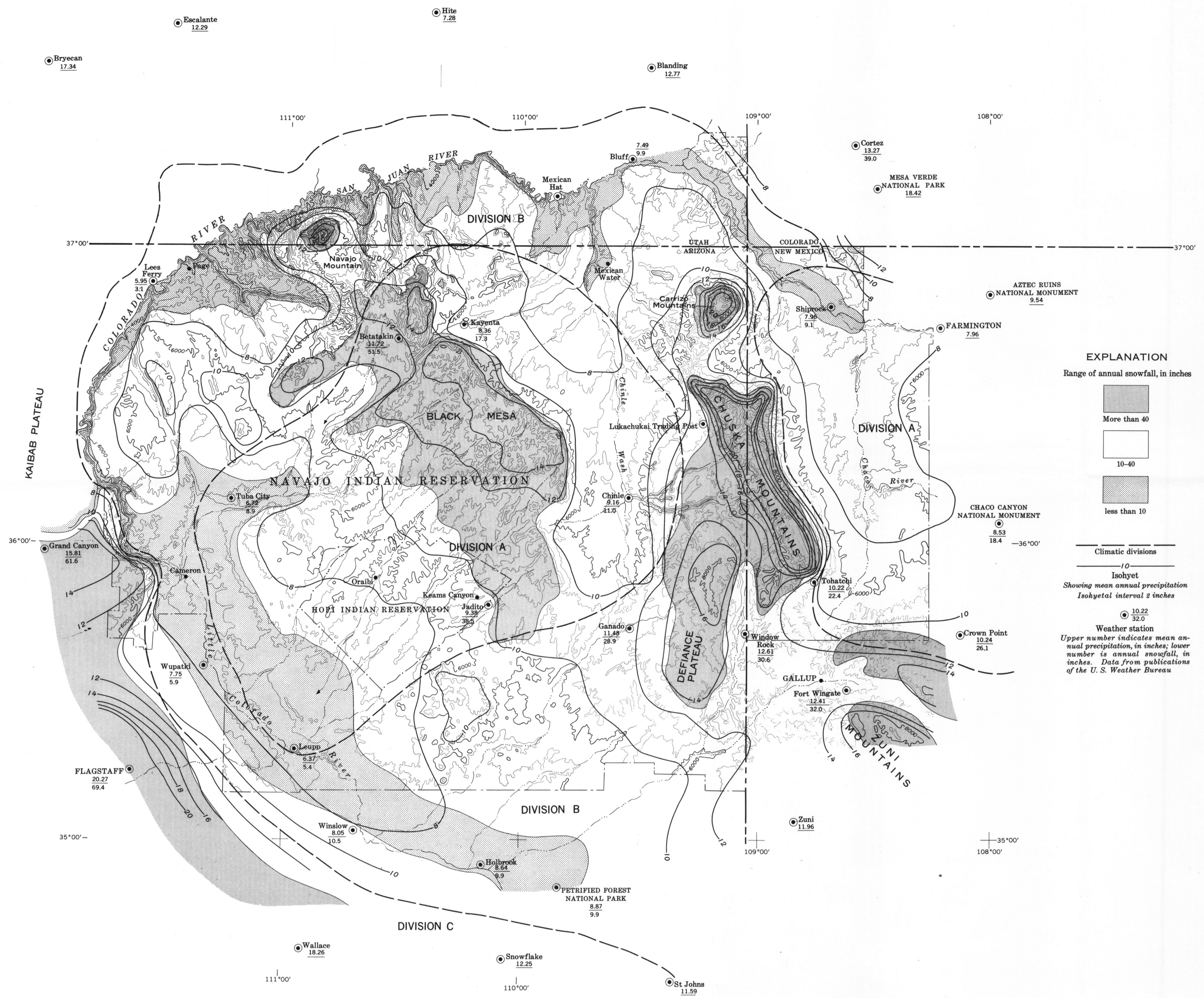
A. ISOHYETAL MAP SHOWING RANGES OF SNOWFALL AND CLIMATIC DIVISIONS
