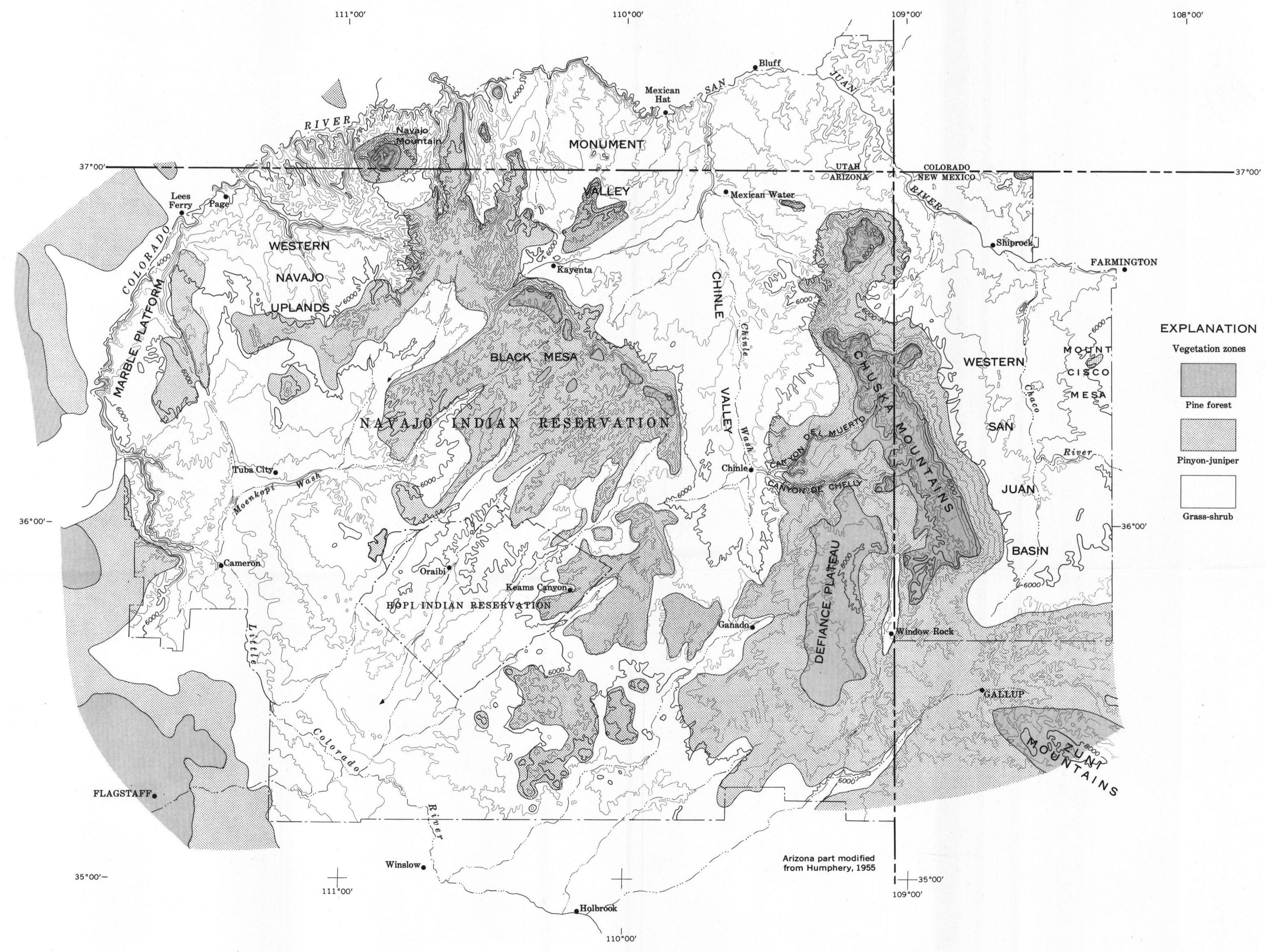
C. MAP SHOWING DISTRIBUTION OF VEGETATION
